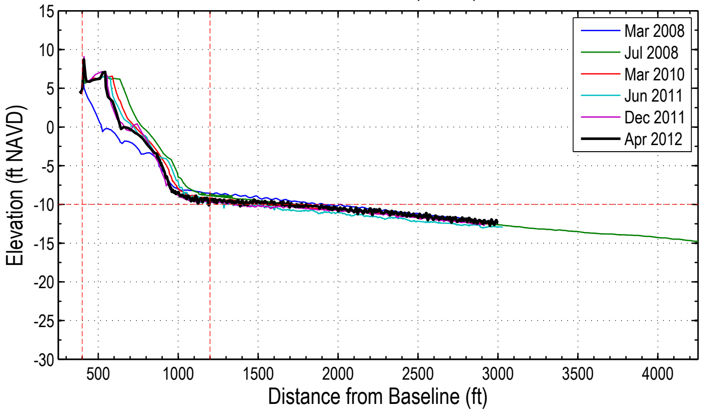
Station: 250+00 (28+00)
