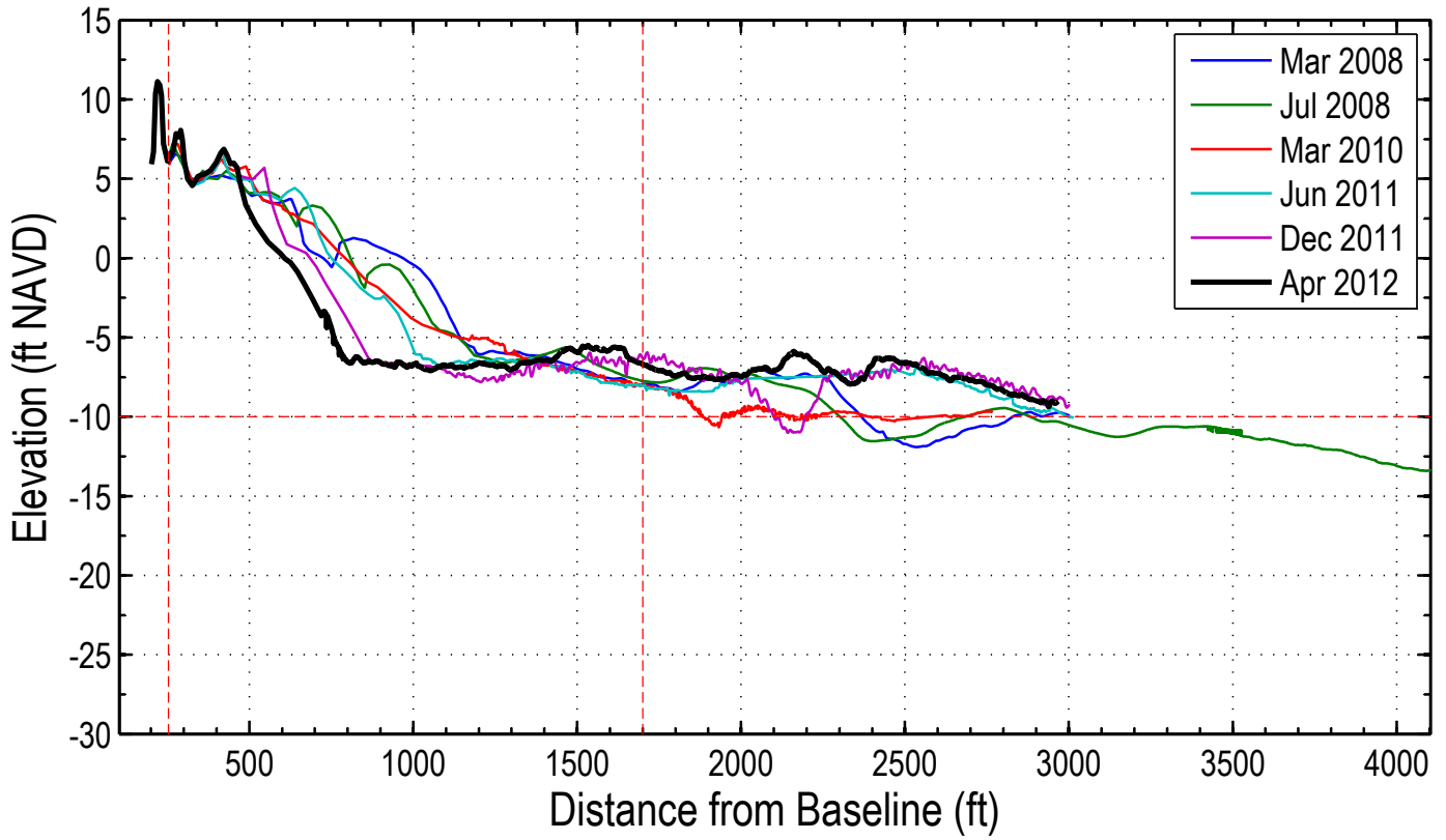
Station: 276+00 (54+00)
