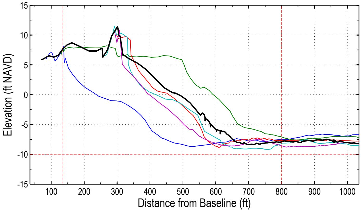
Station: 318+00 (96+00)
