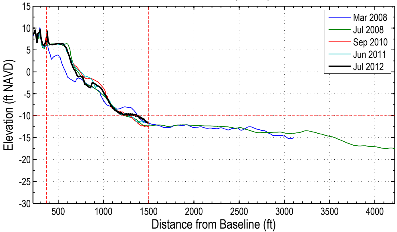
Station: 232+00 (10+00)
