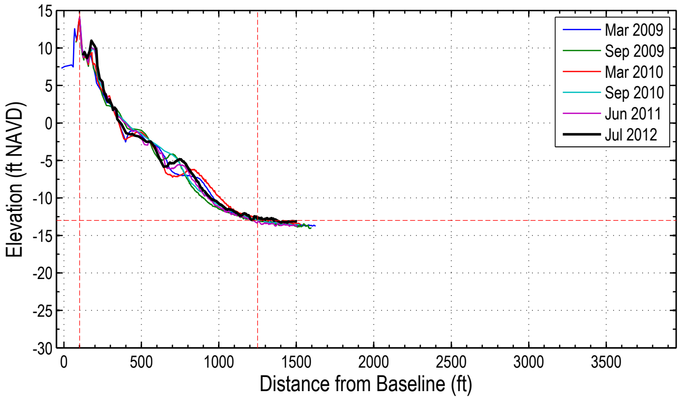
Station: 140+00
