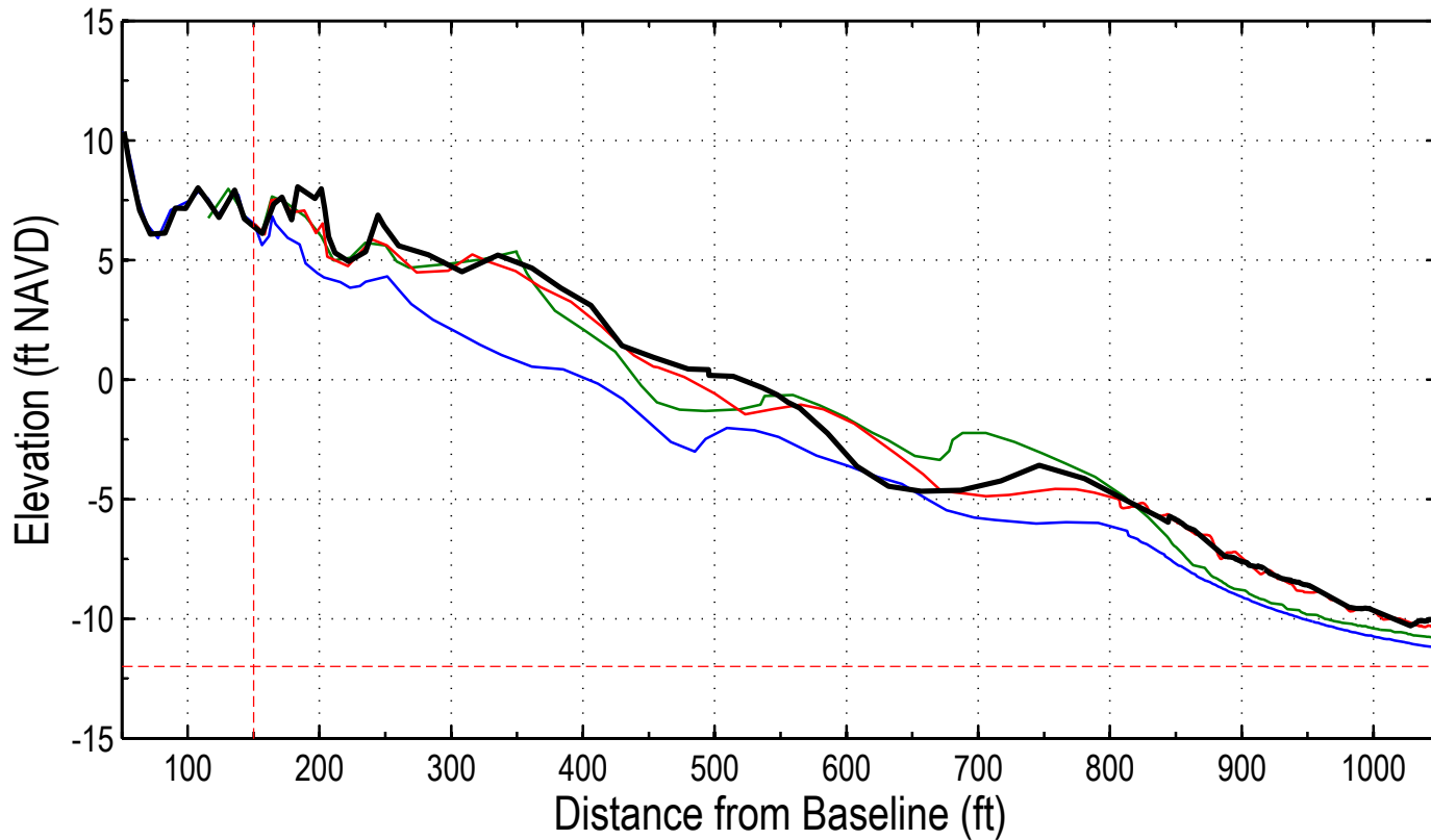
Station: 206+00 (-16+00)
