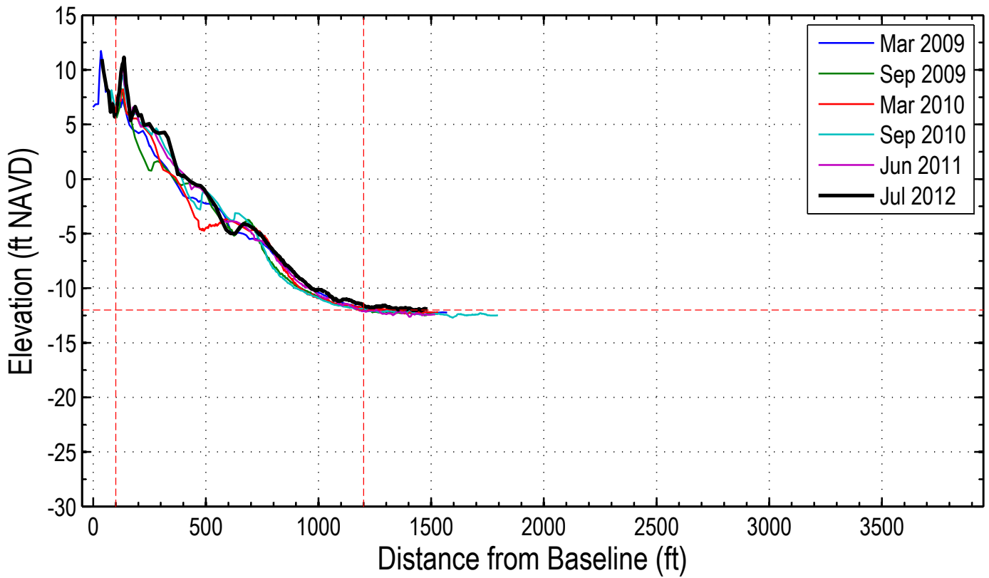
Station: 200+00
