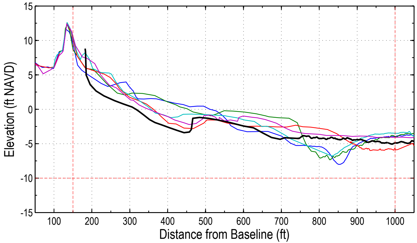
Station: 8+00
