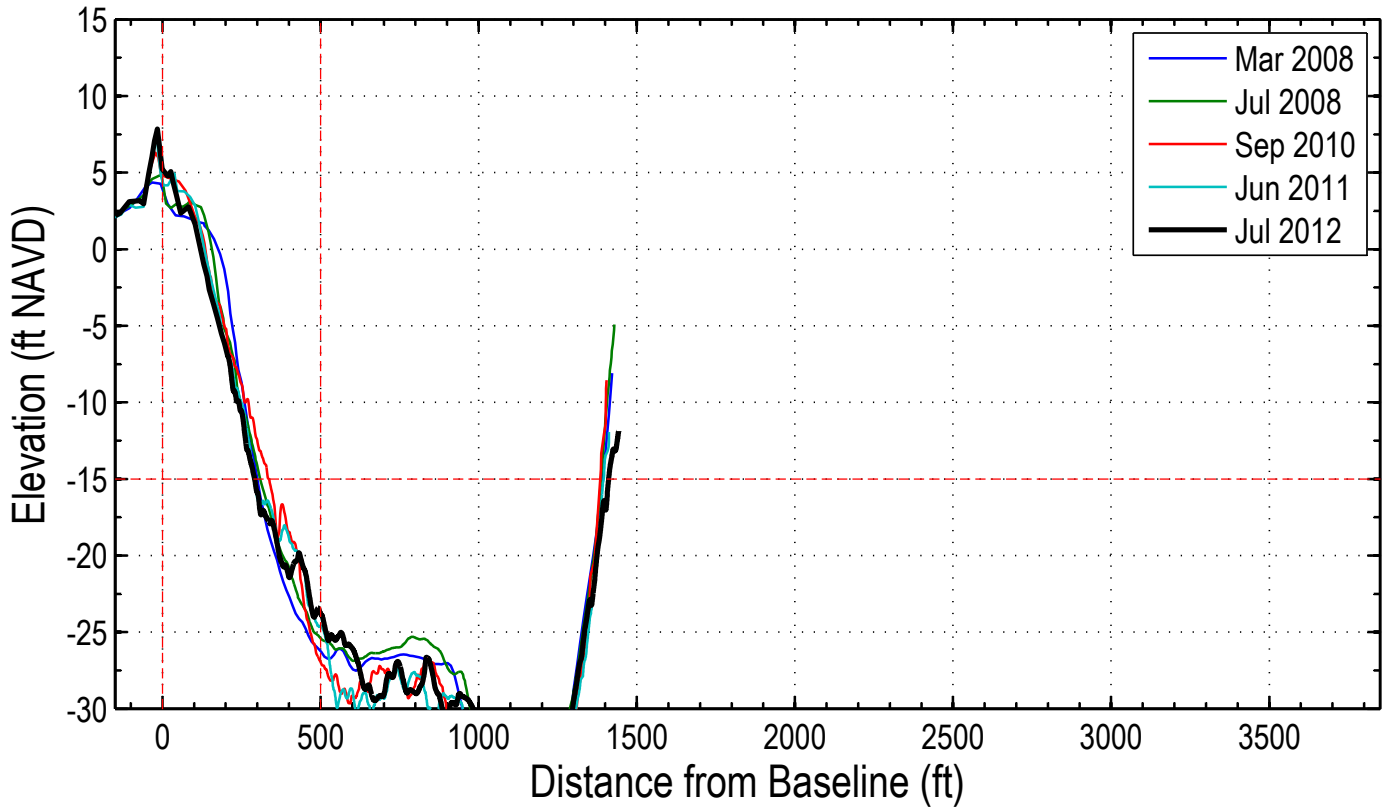
Station: 364+00 (142+00)
