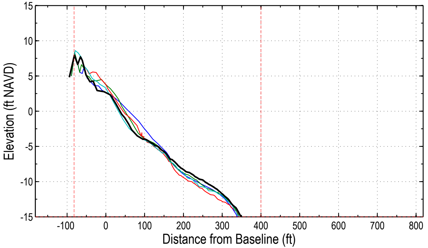
Station: 350+00 (128+00)
