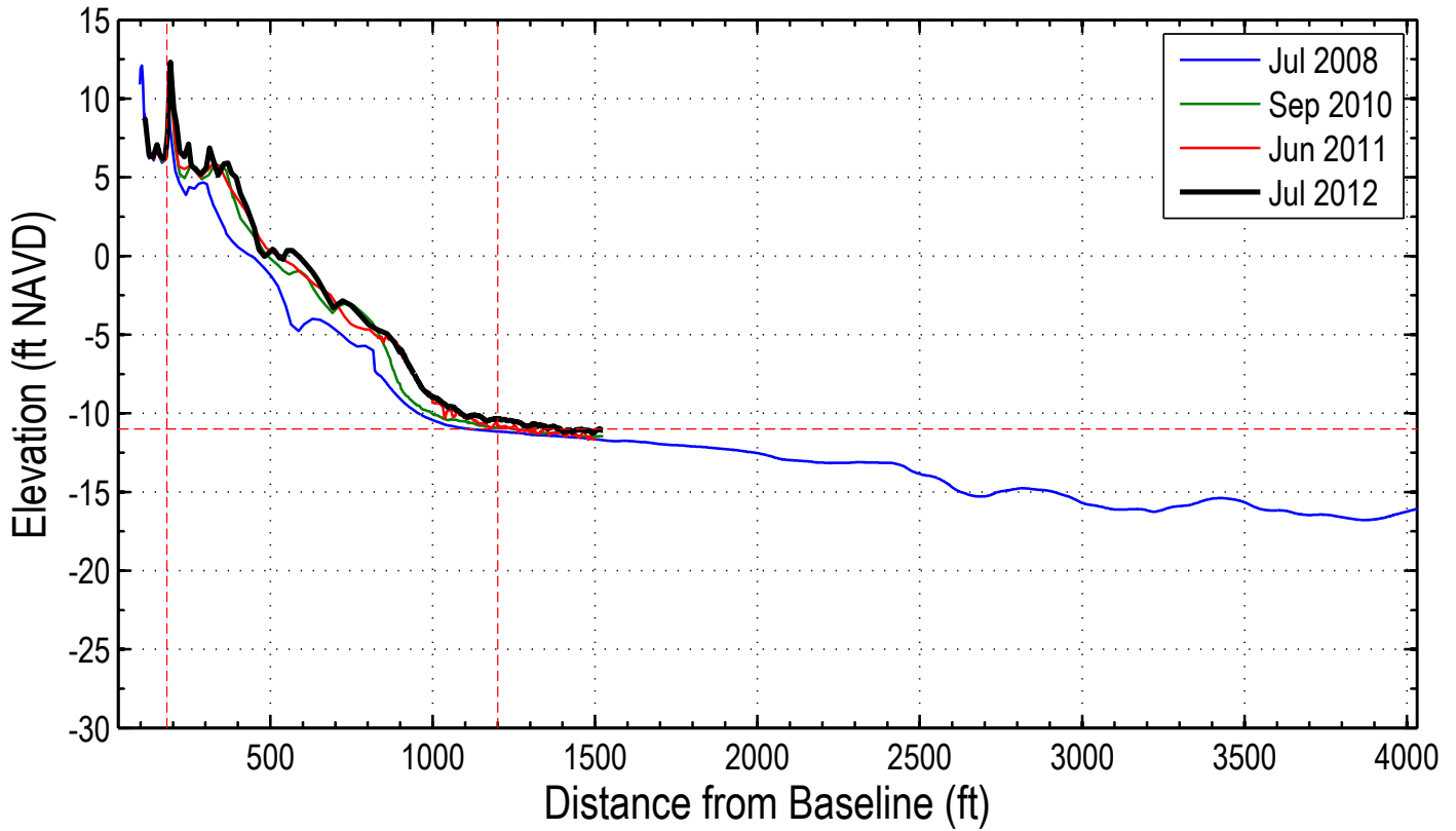
Station: 214+00 (-8+00)
