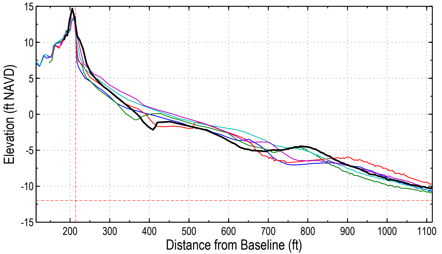
Station: 30+00
