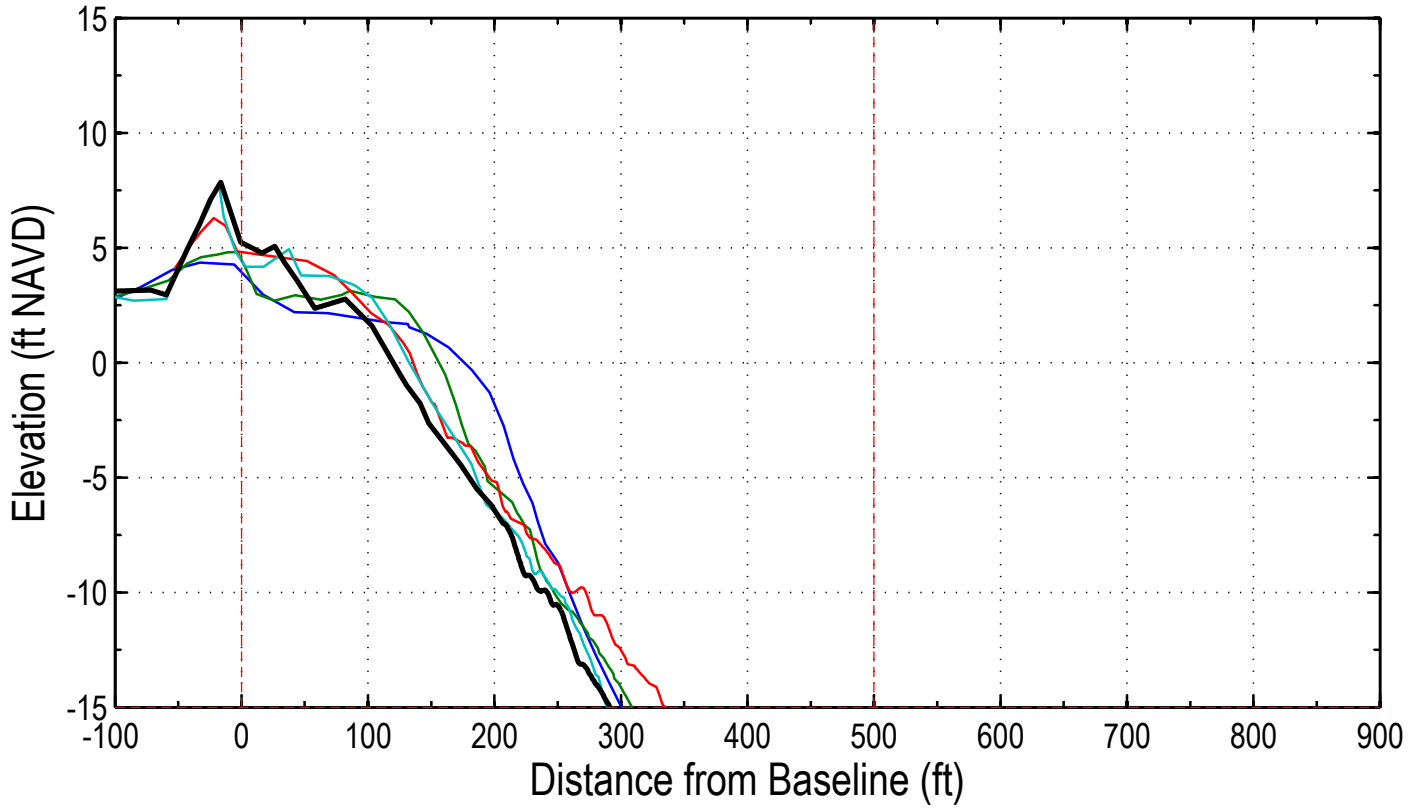
Station: 364+00 (142+00)
