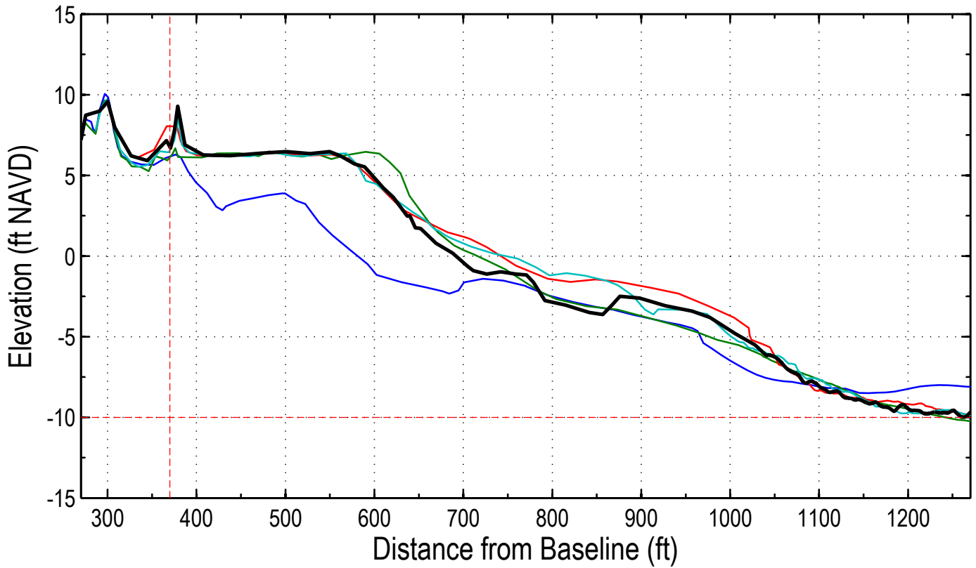
Station: 232+00 (10+00)
