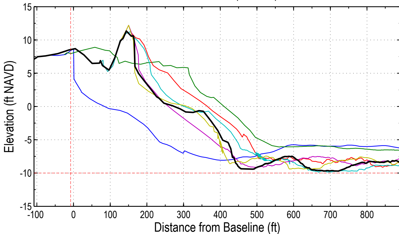
Station: 324+00 (102+00)
