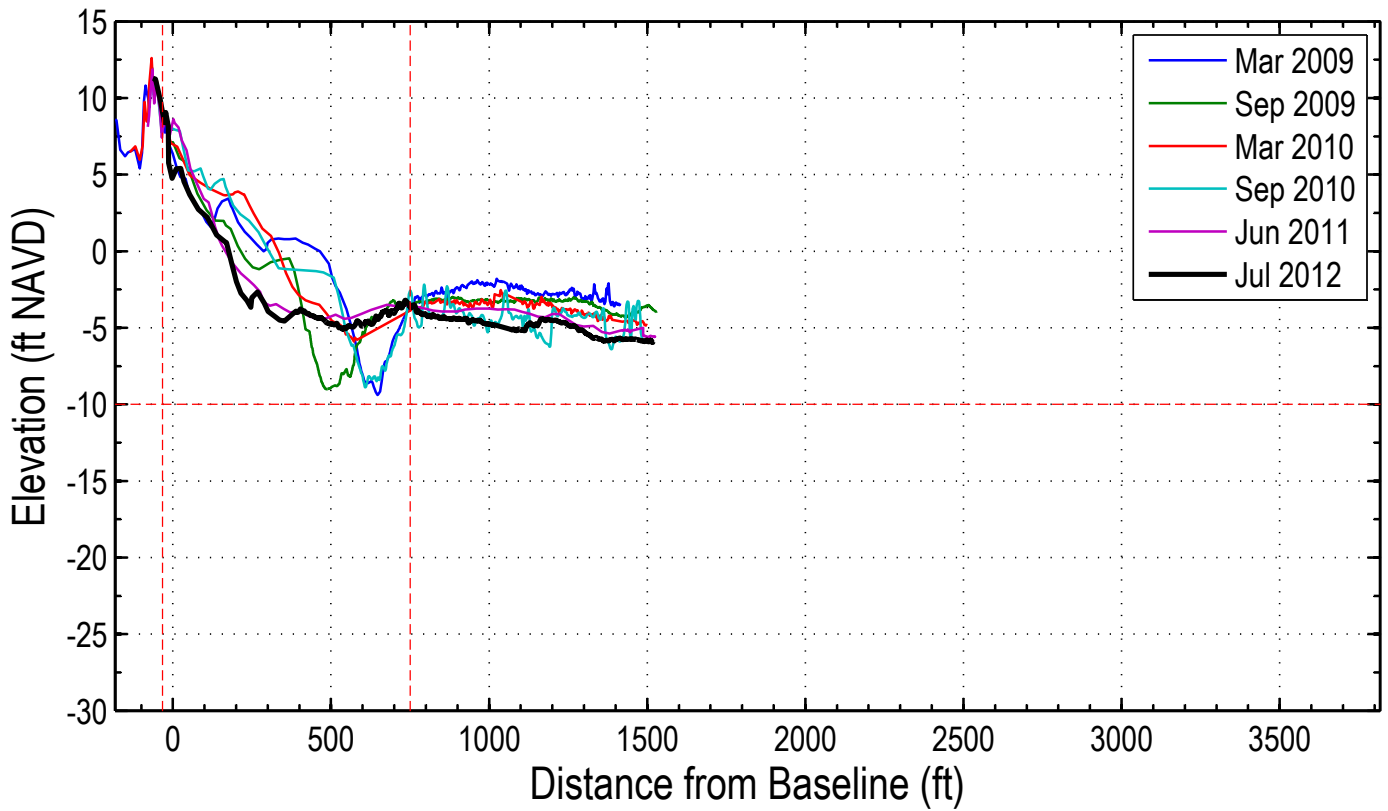
Station: 4+00
