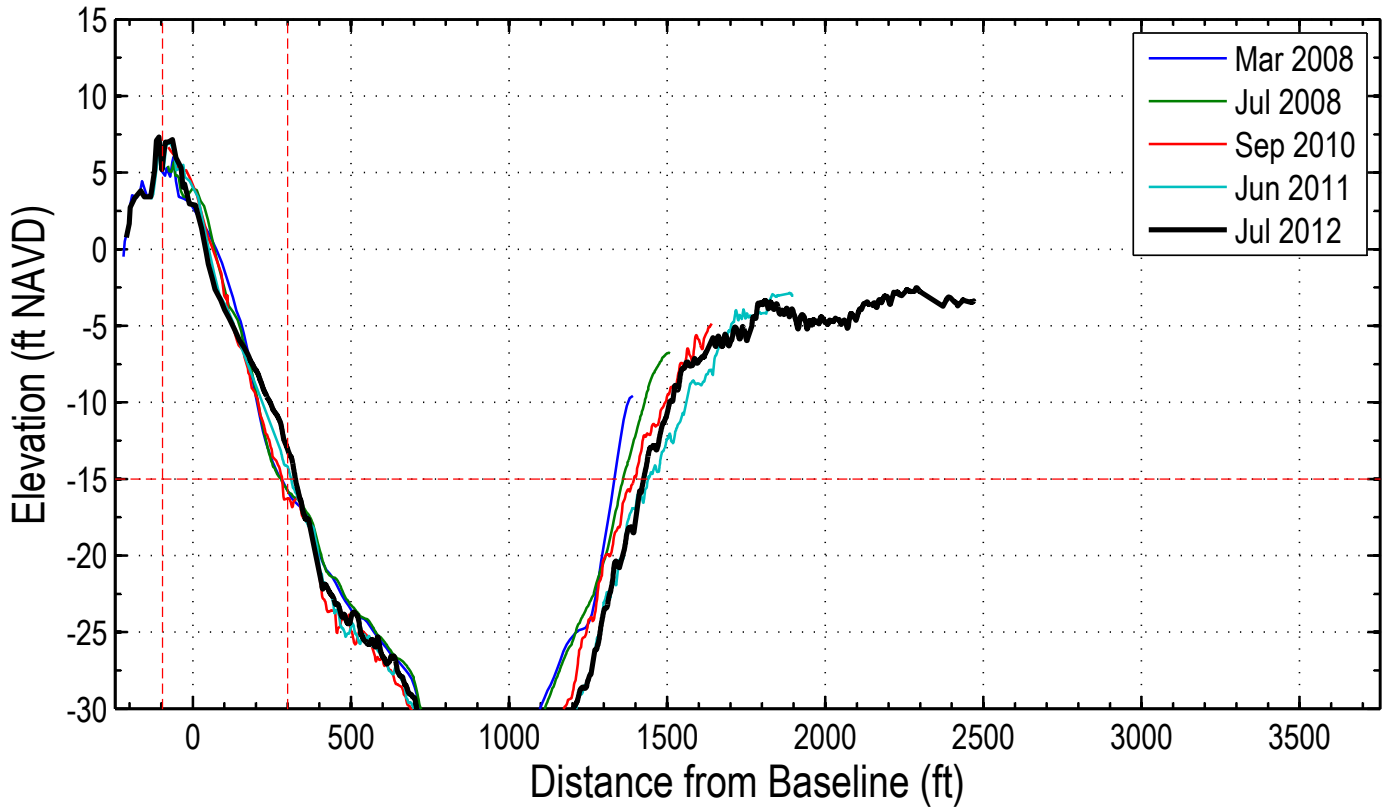
Station: 354+00 (132+00)
