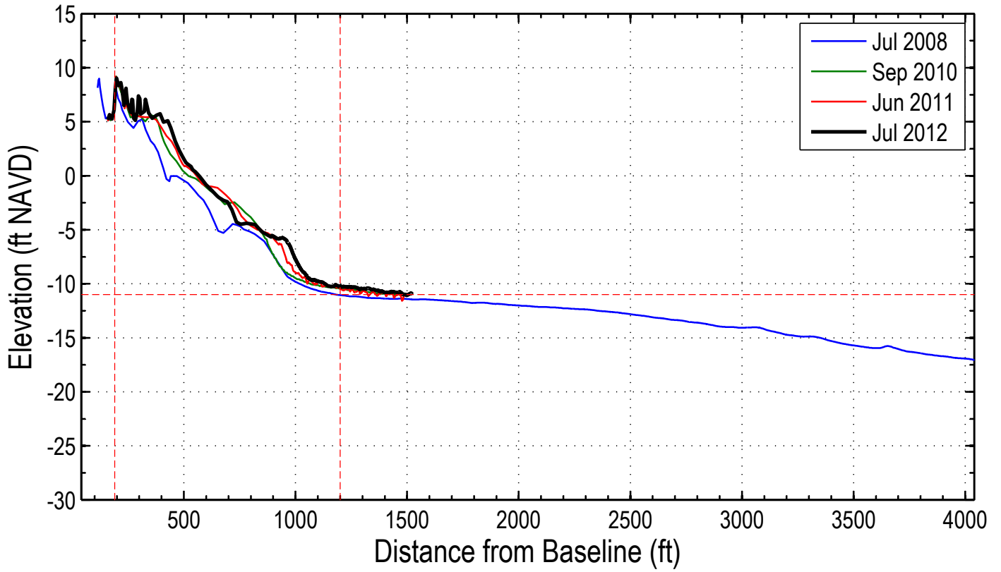
Station: 218+00 (-4+00)
