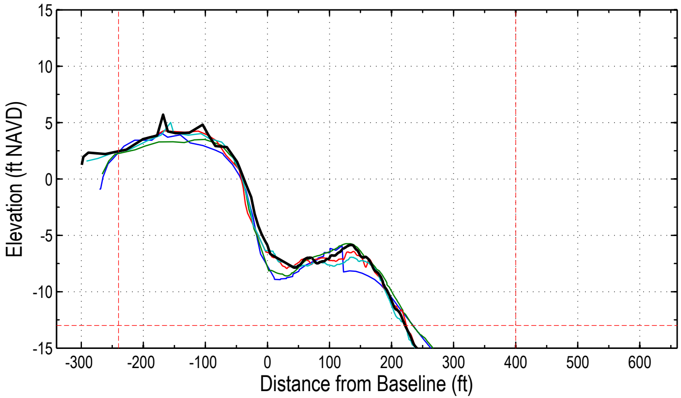
Station: 368+00 (146+00)
