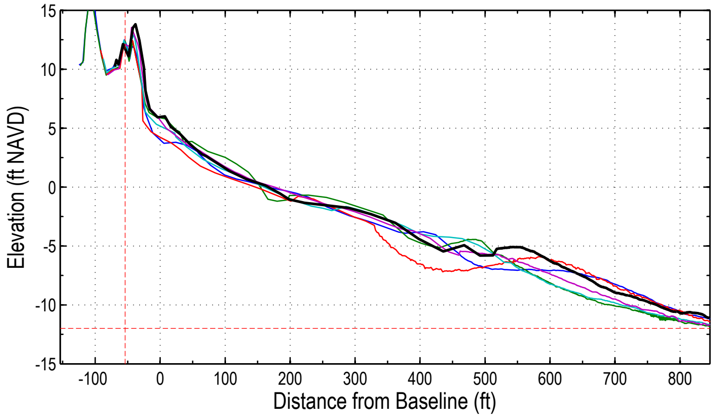
Station: 70+00
