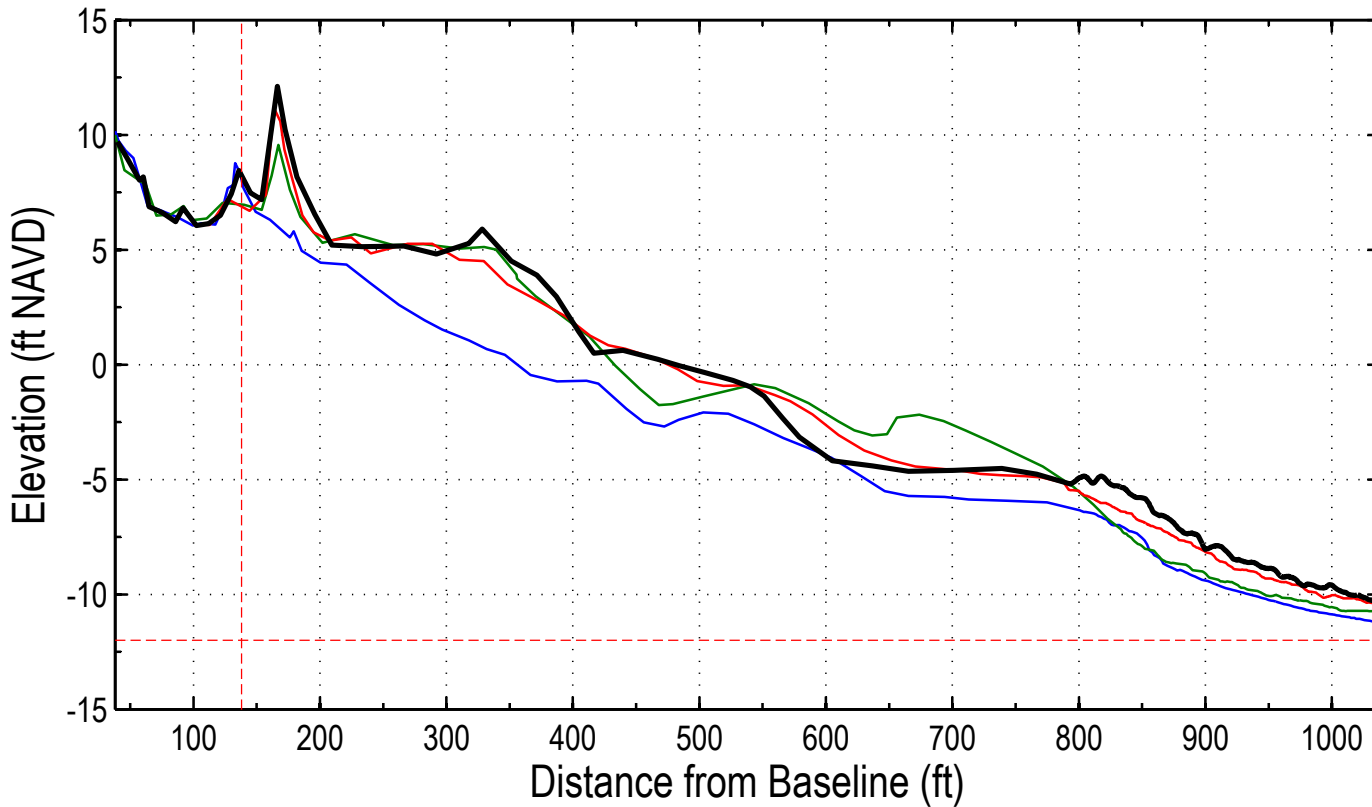
Station: 204+00 (-18+00)
