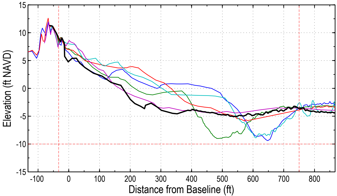
Station: 4+00
