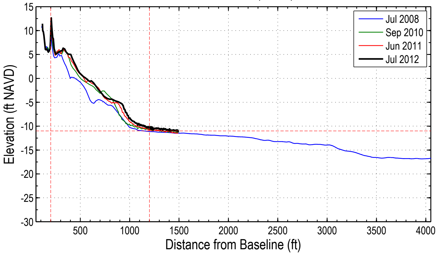
Station: 216+00 (-6+00)
