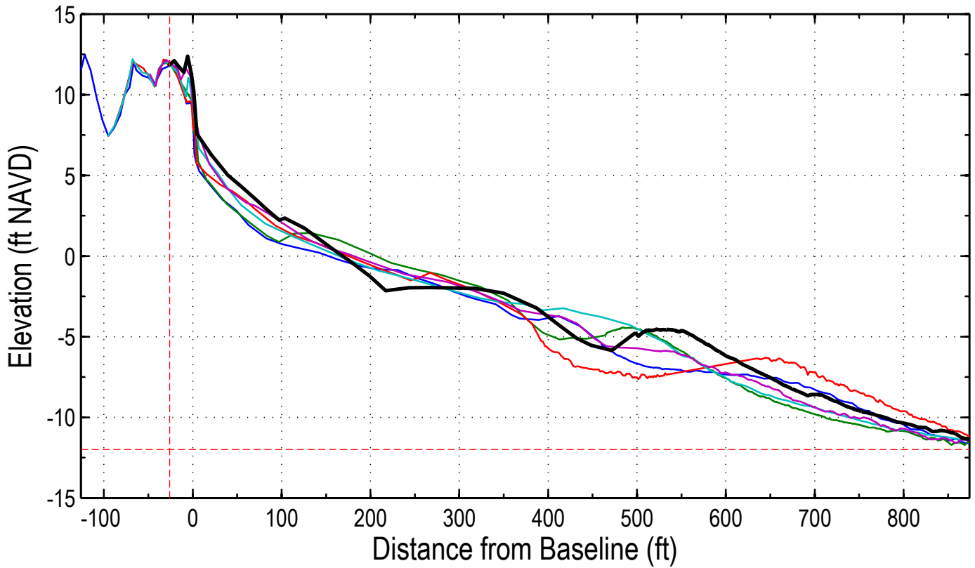
Station: 60+00
