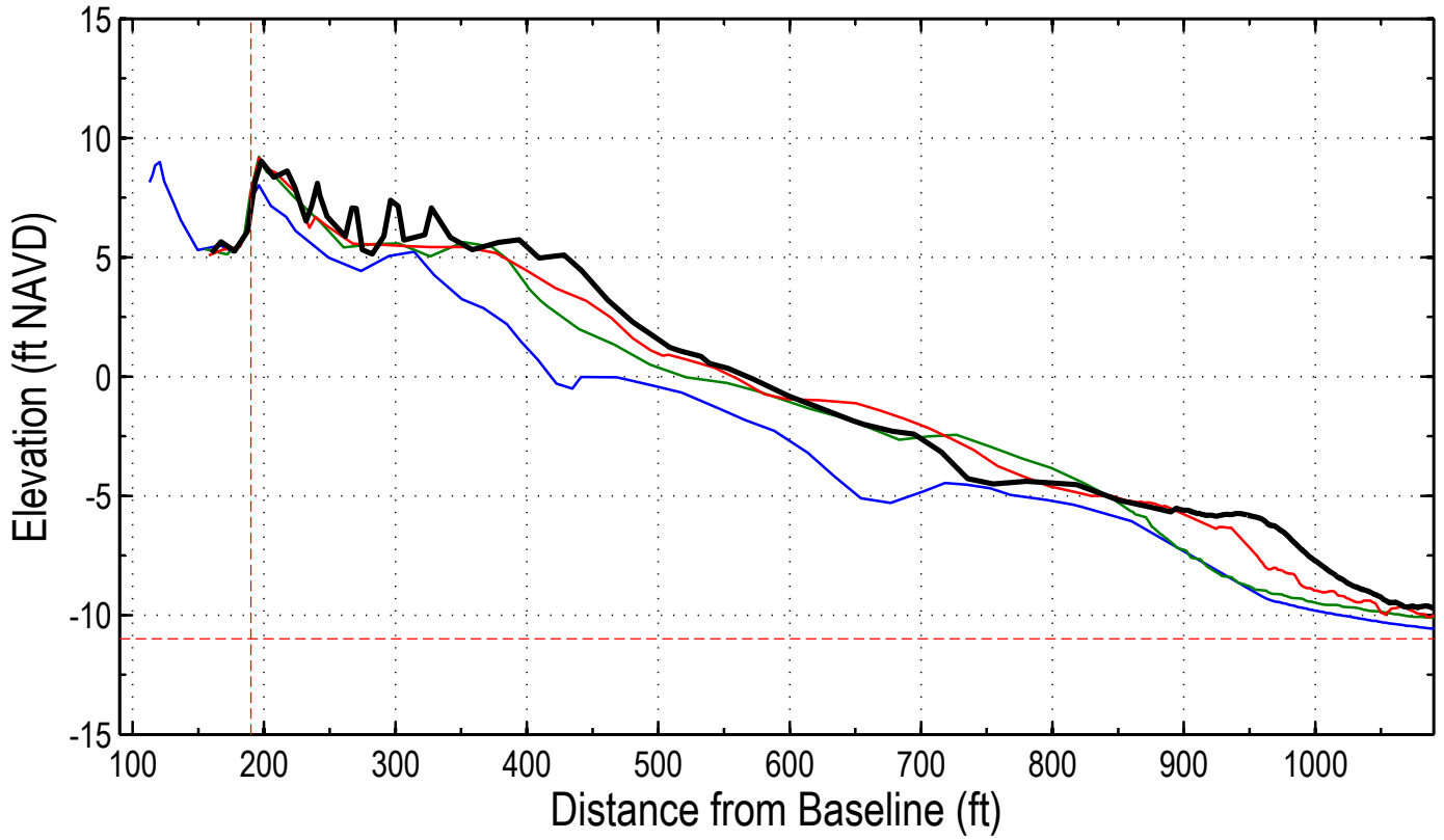
Station: 218+00 (-4+00)
