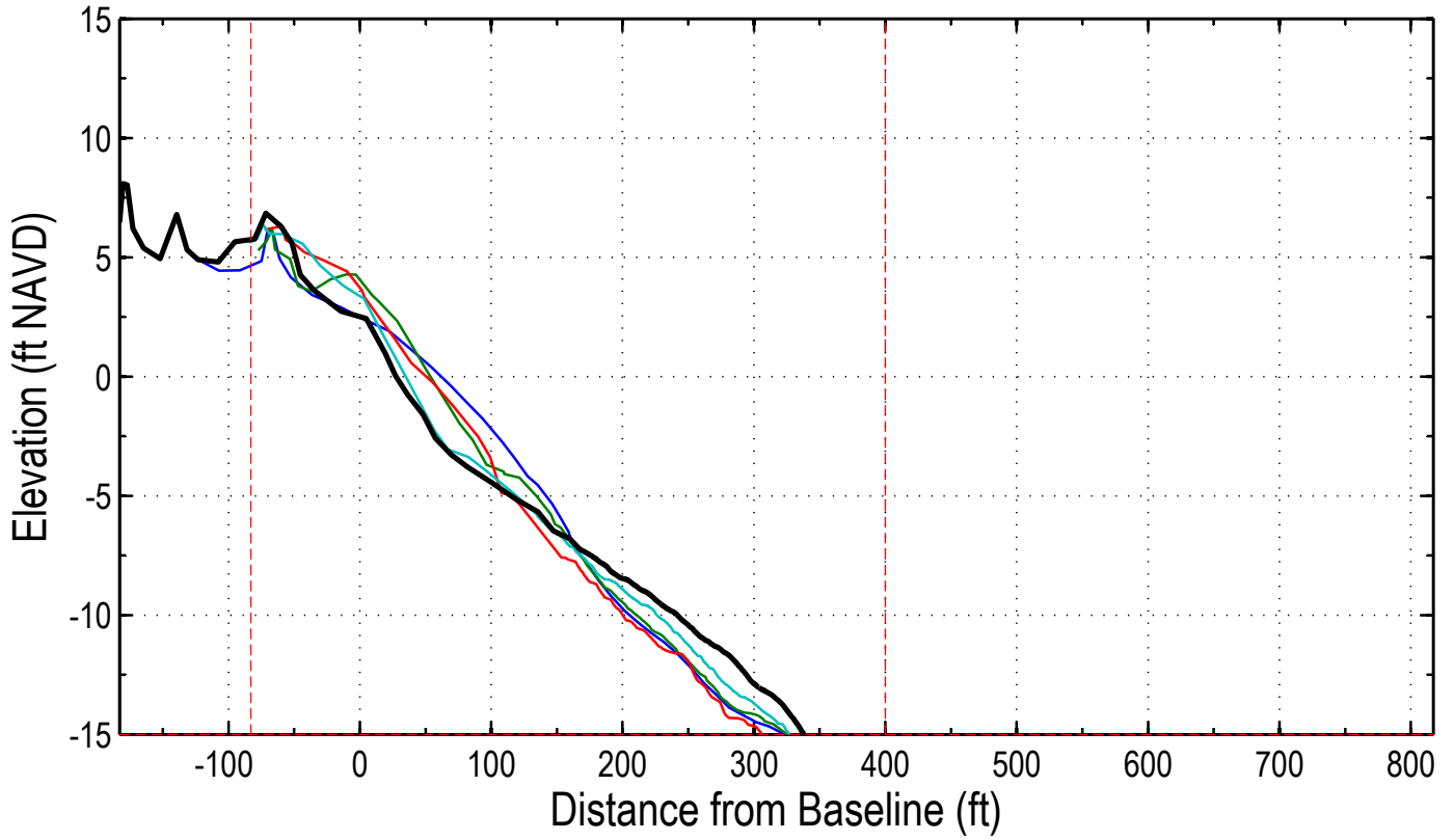
Station: 352+00 (130+00)
