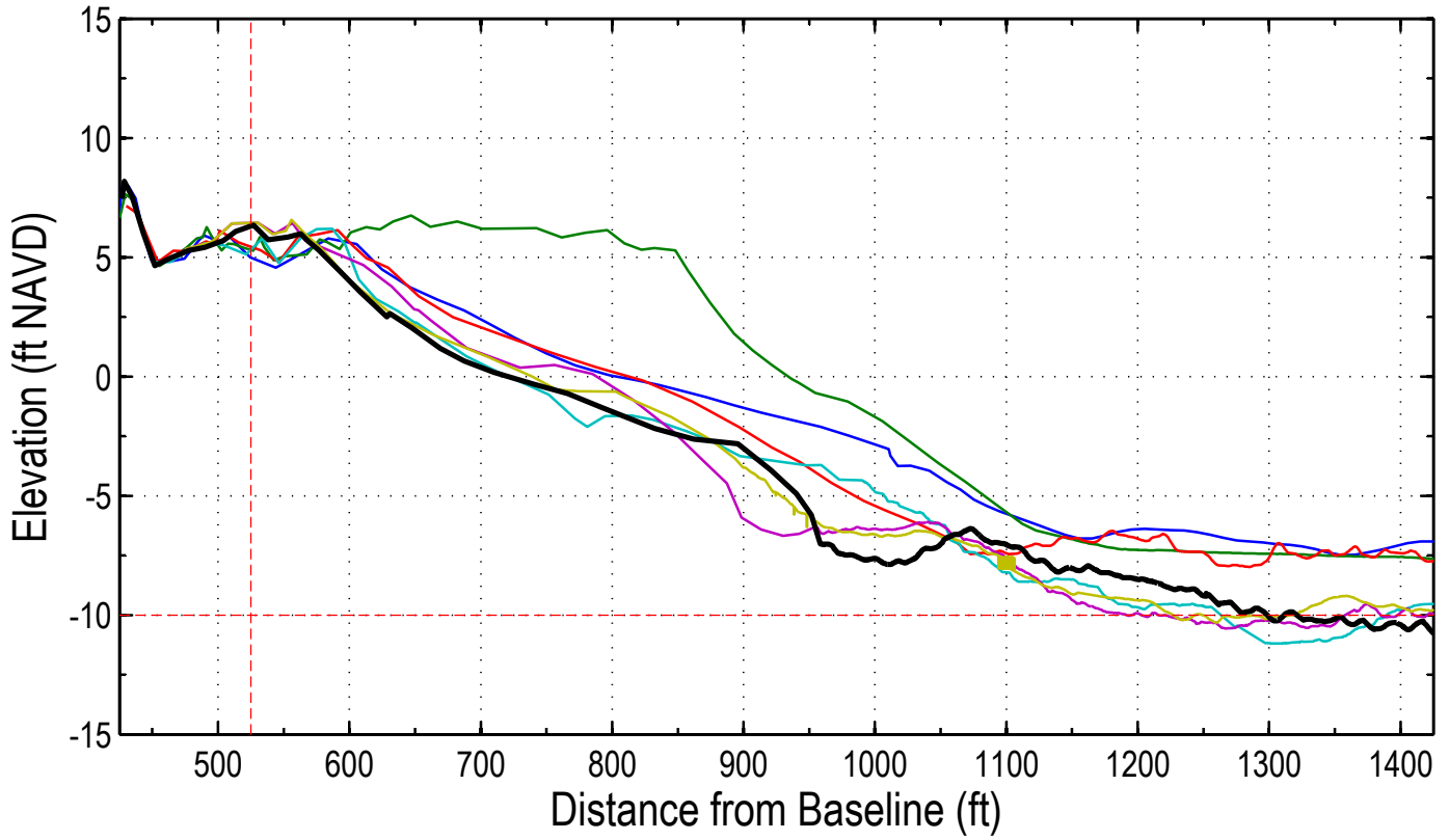
Station: 264+00 (42+00)
