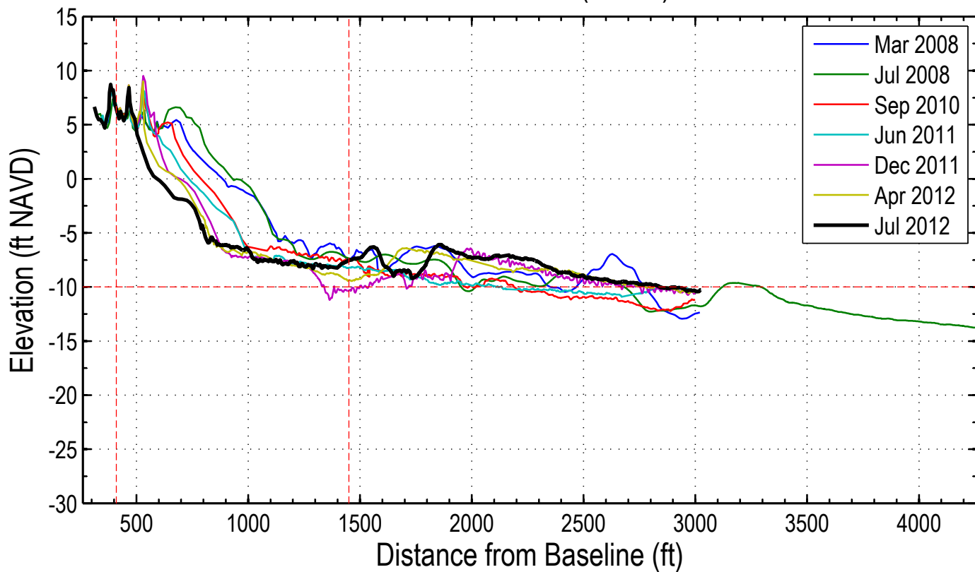
Station: 272+00 (50+00)
