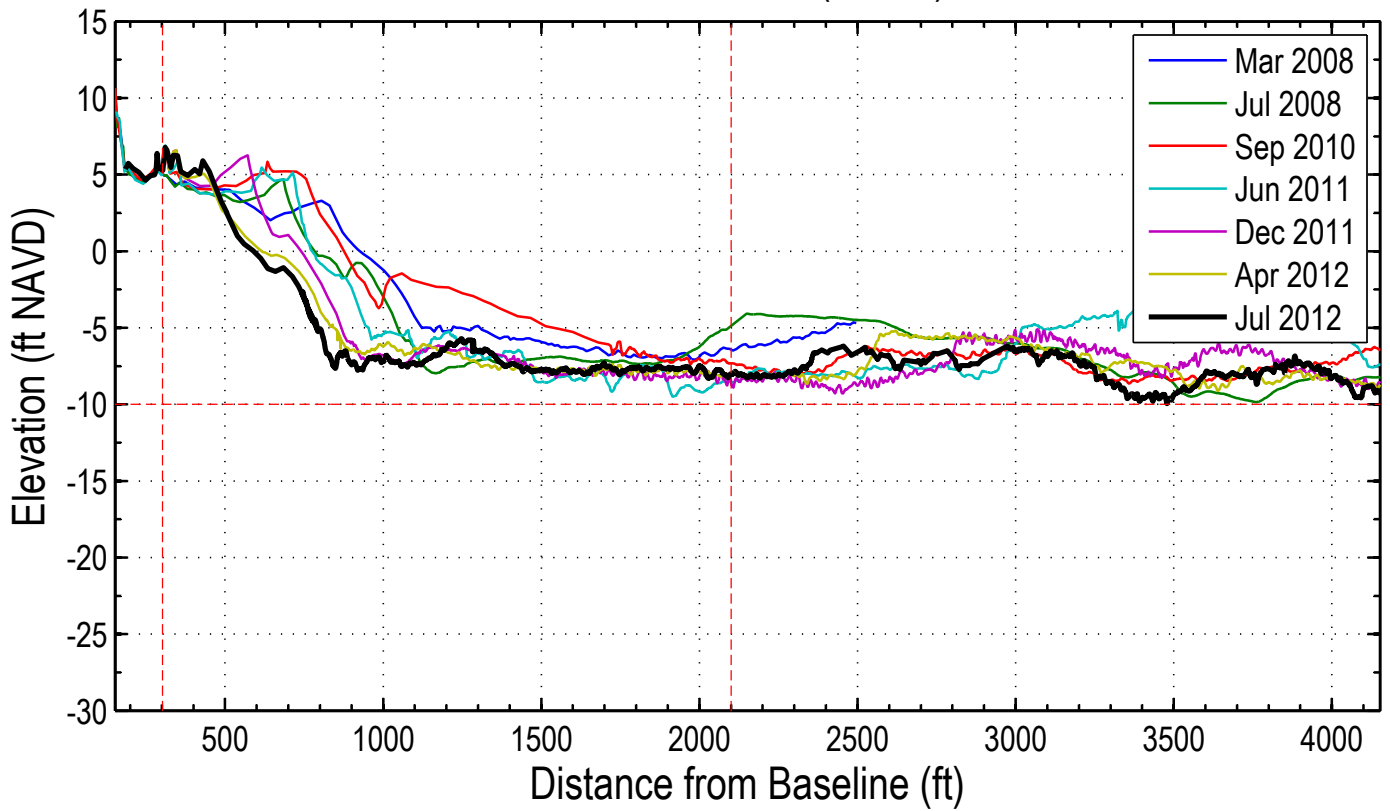
Station: 282+00 (60+00)
