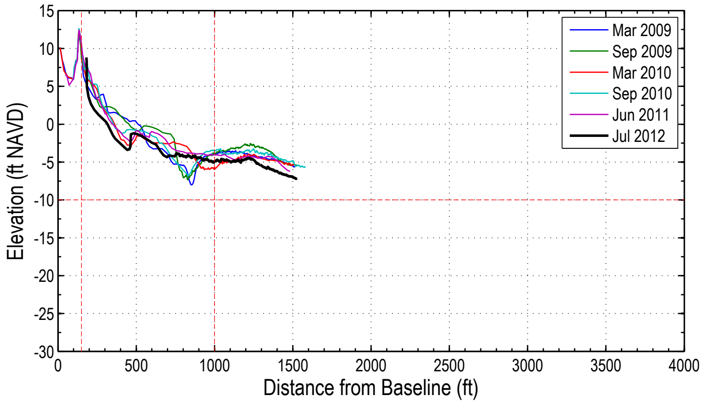
Station: 8+00
