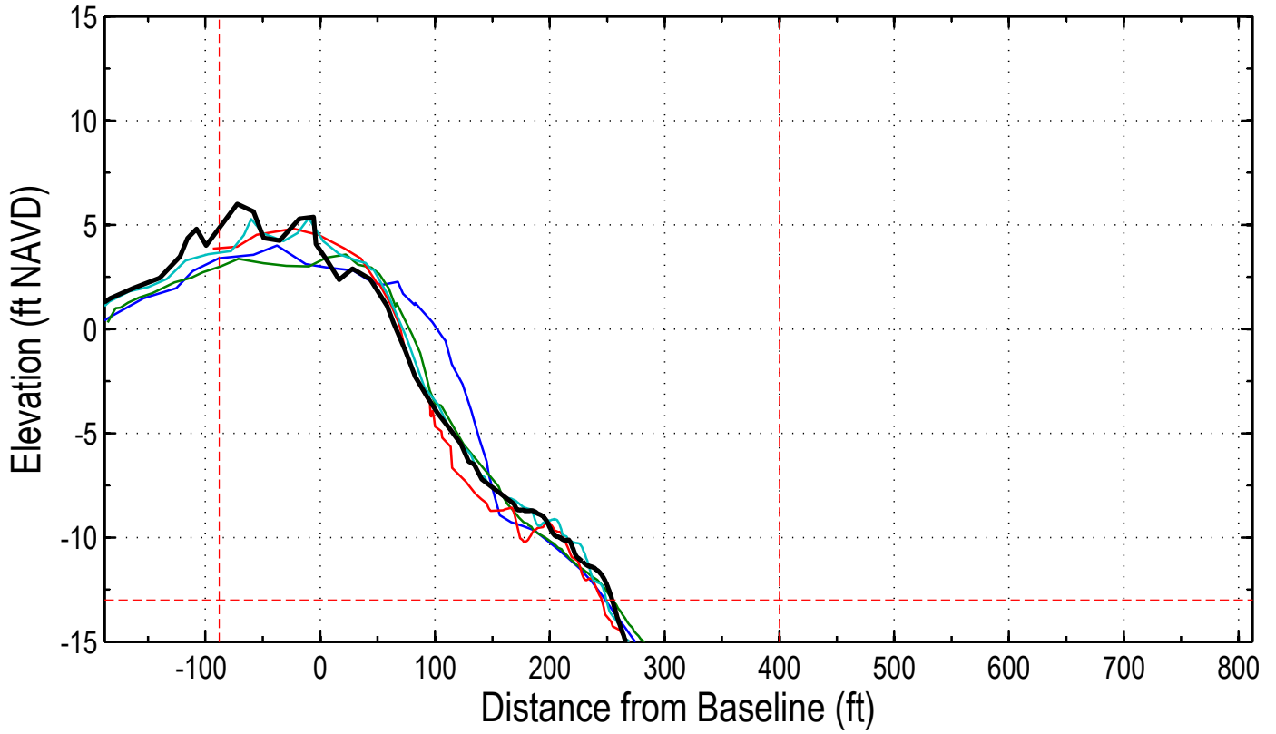
Station: 366+00 (144+00)
