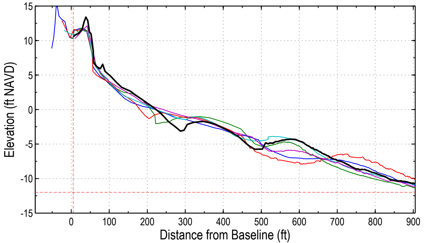
Station: 50+00
