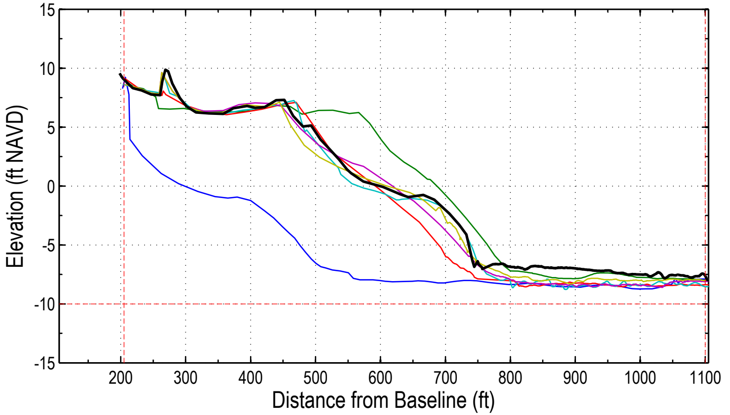
Station: 304+00 (82+00)
