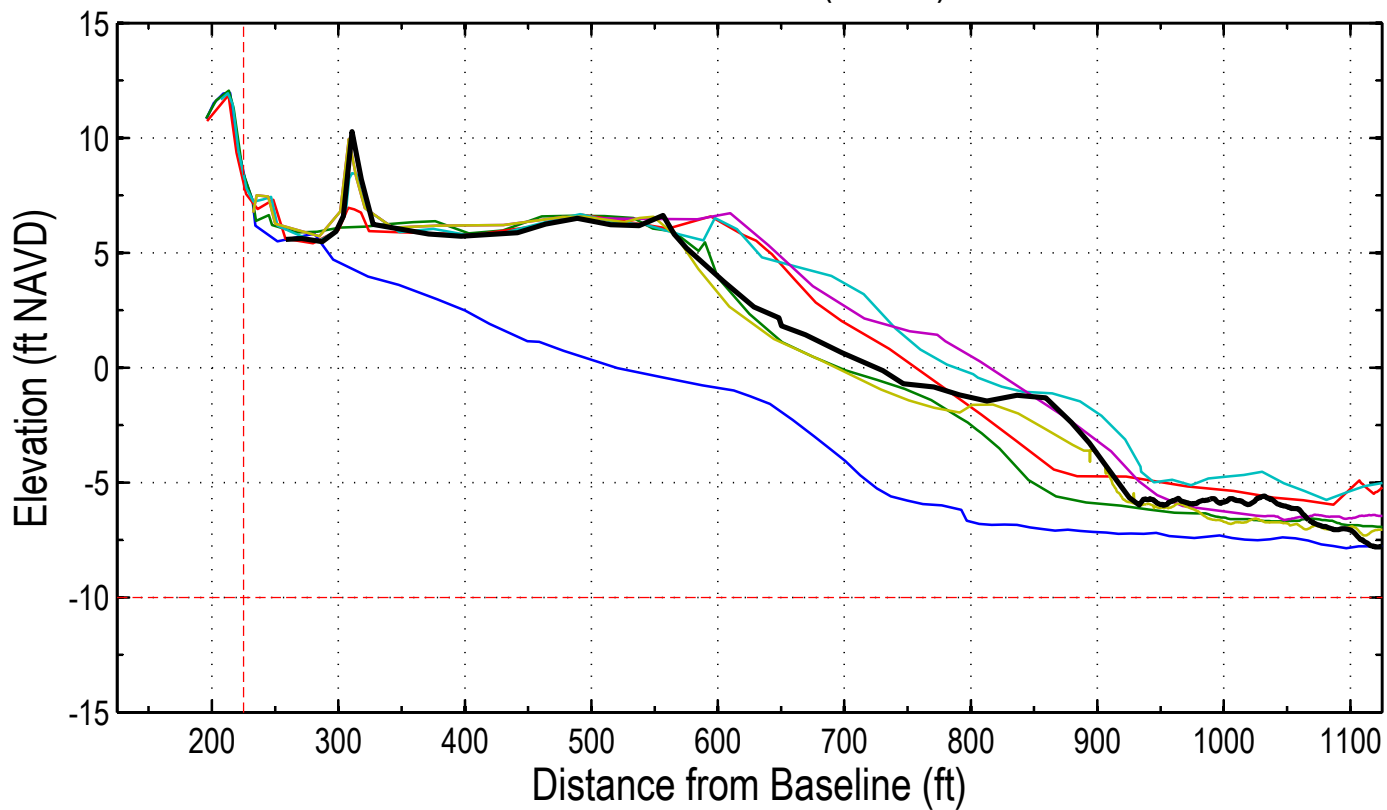
Station: 290+00 (68+00)
