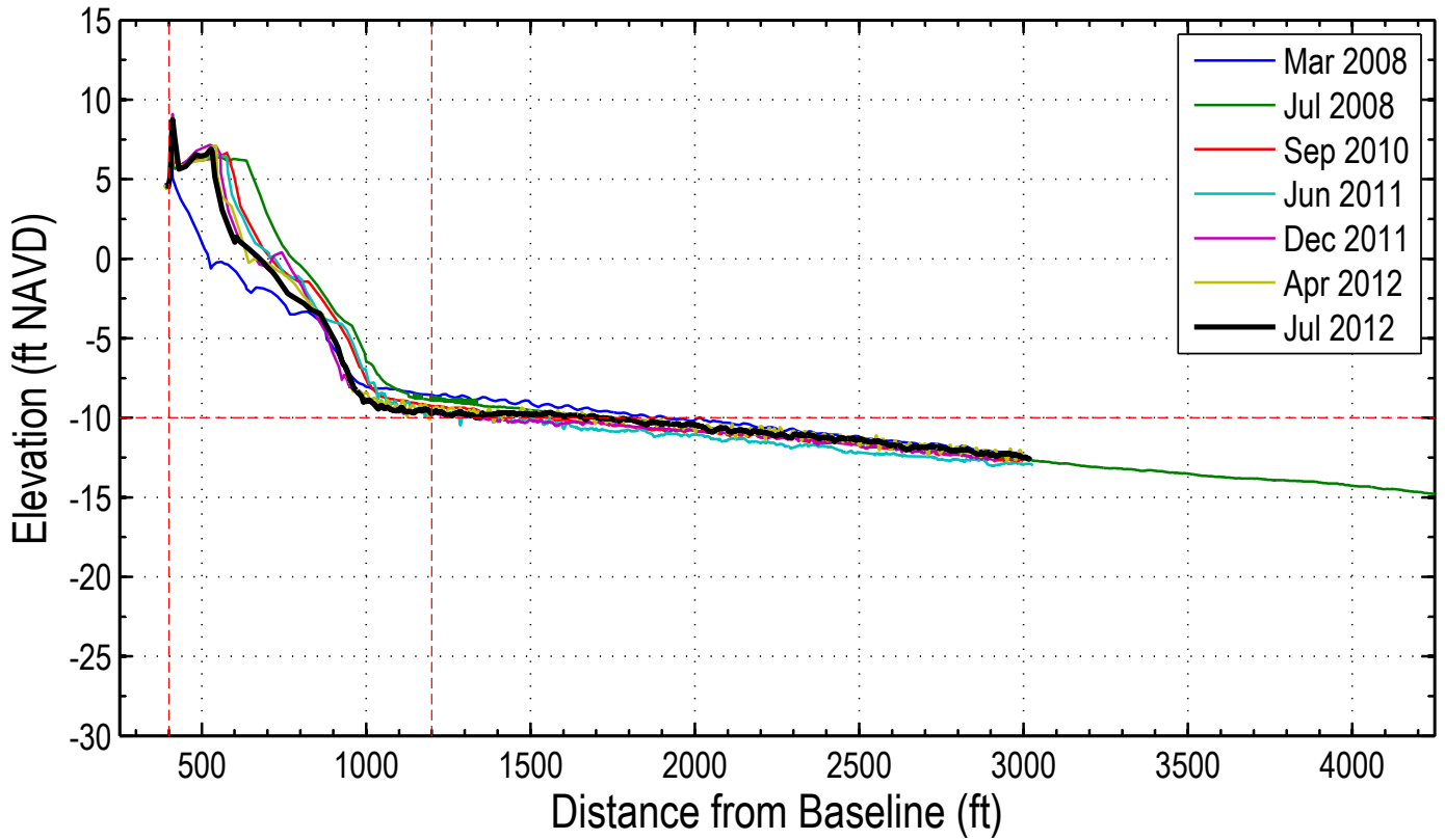
Station: 250+00 (28+00)
