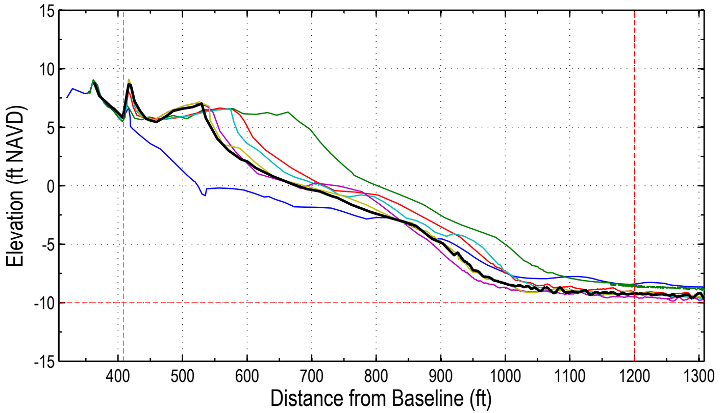
Station: 252+00 (30+00)
