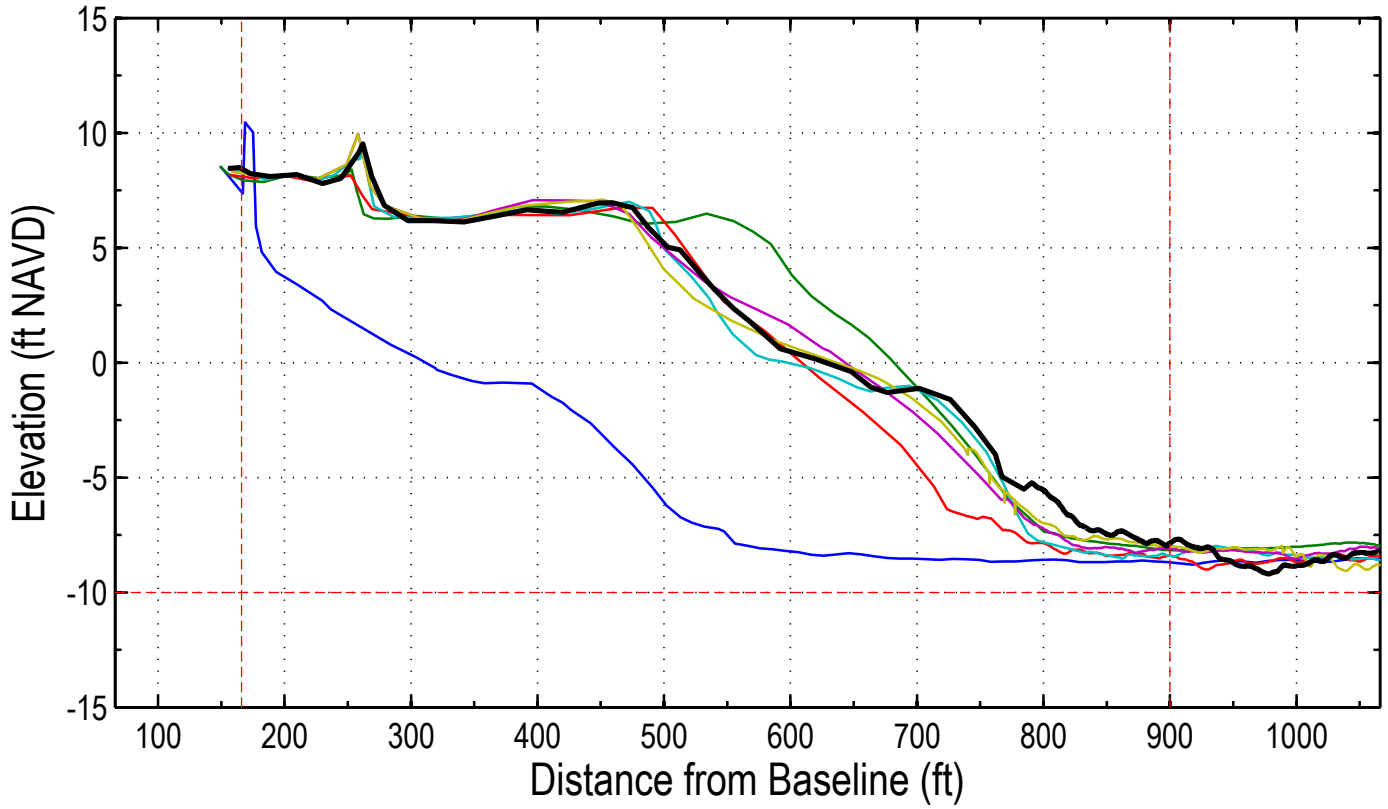
Station: 302+00 (80+00)
