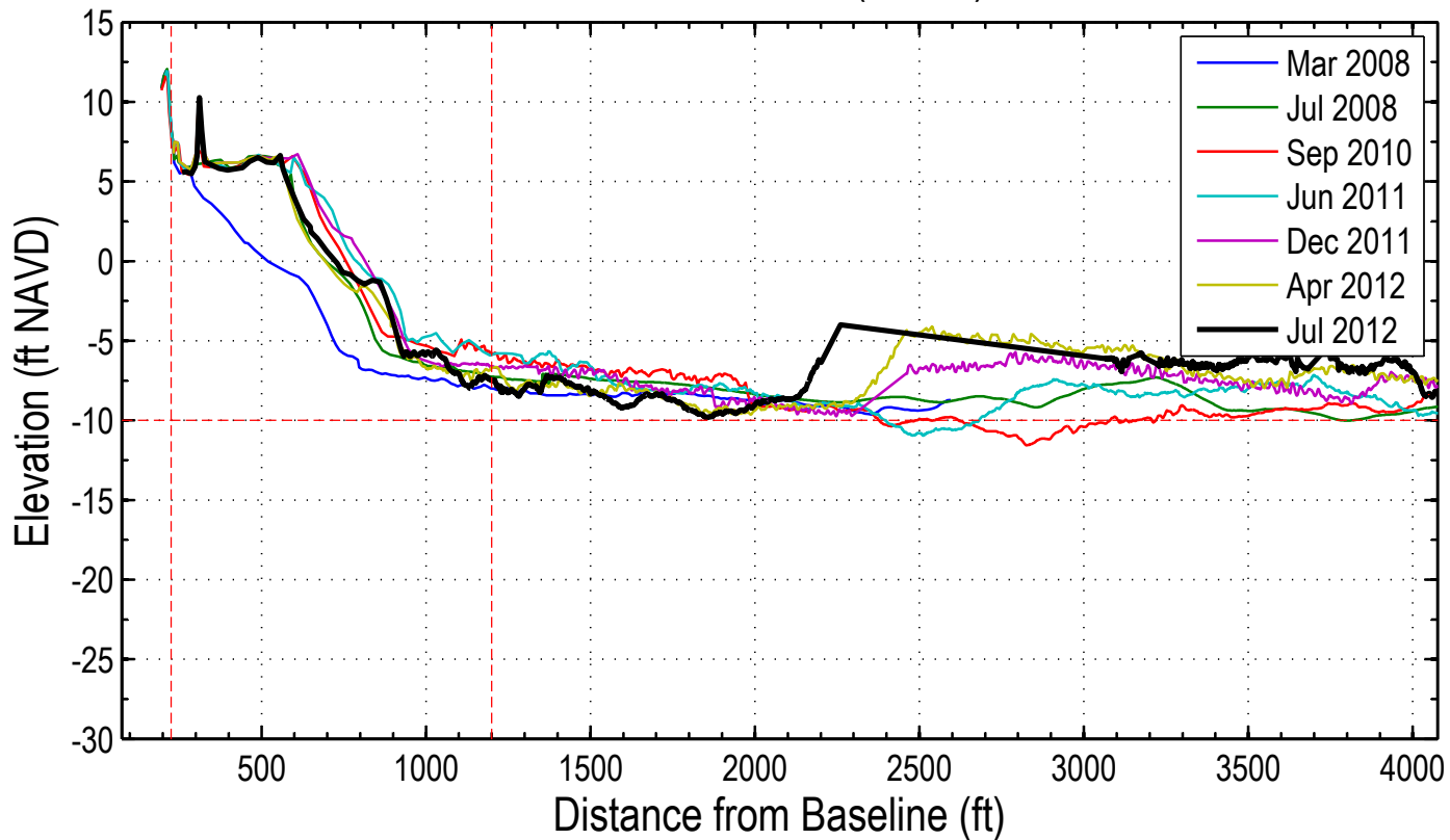
Station: 290+00 (68+00)
