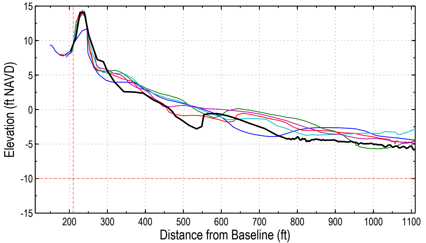
Station: 12+00
