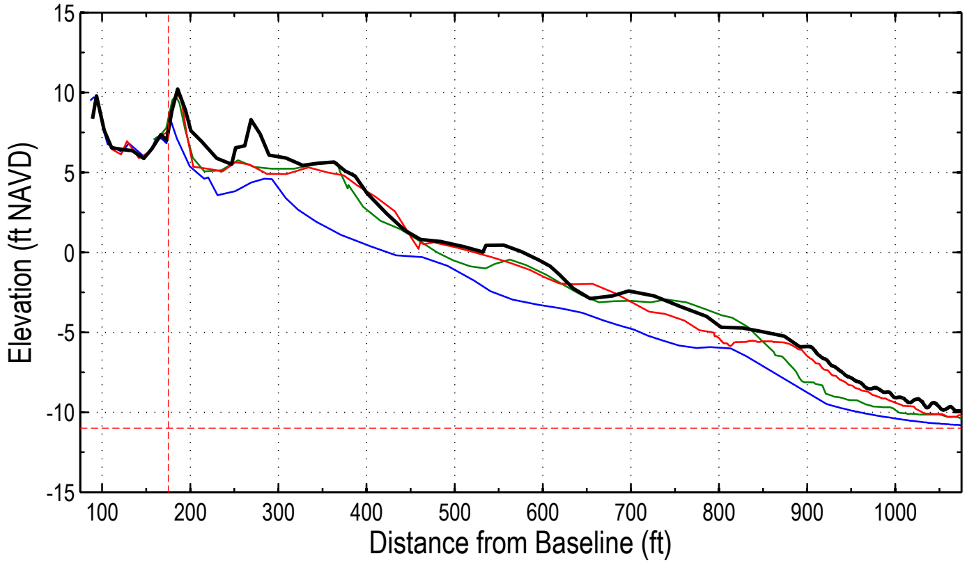
Station: 212+00 (-10+00)
