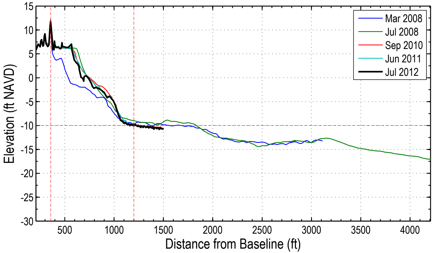
Station: 236+00 (14+00)
