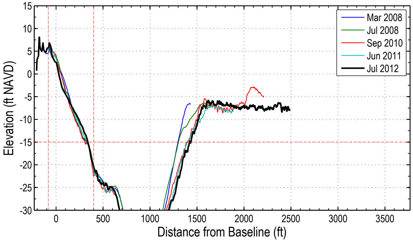
Station: 352+00 (130+00)
