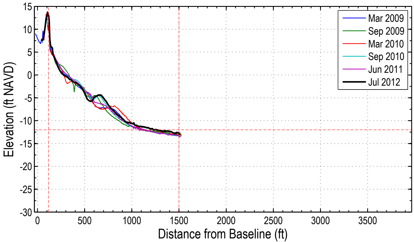
Station: 40+00
