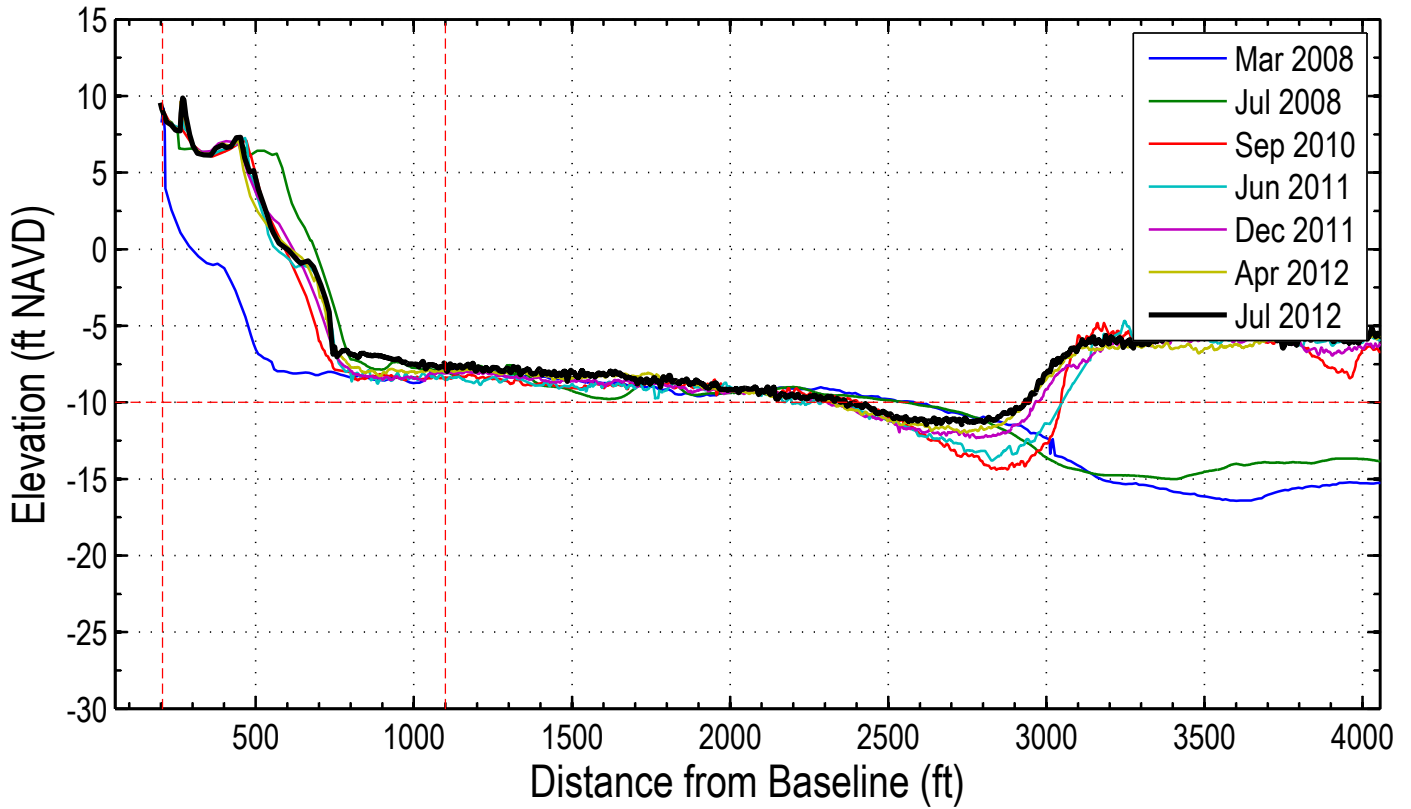
Station: 304+00 (82+00)
