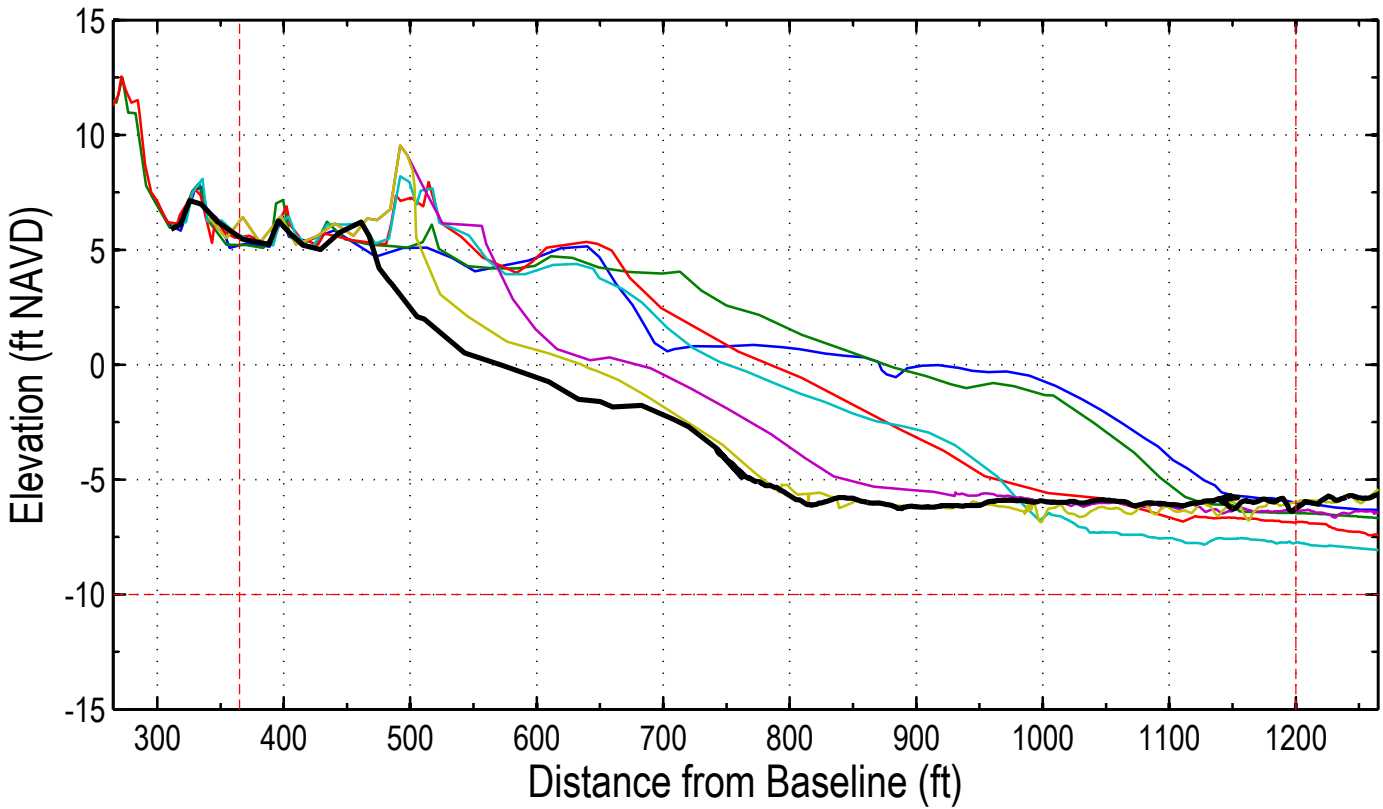
Station: 274+00 (52+00)
