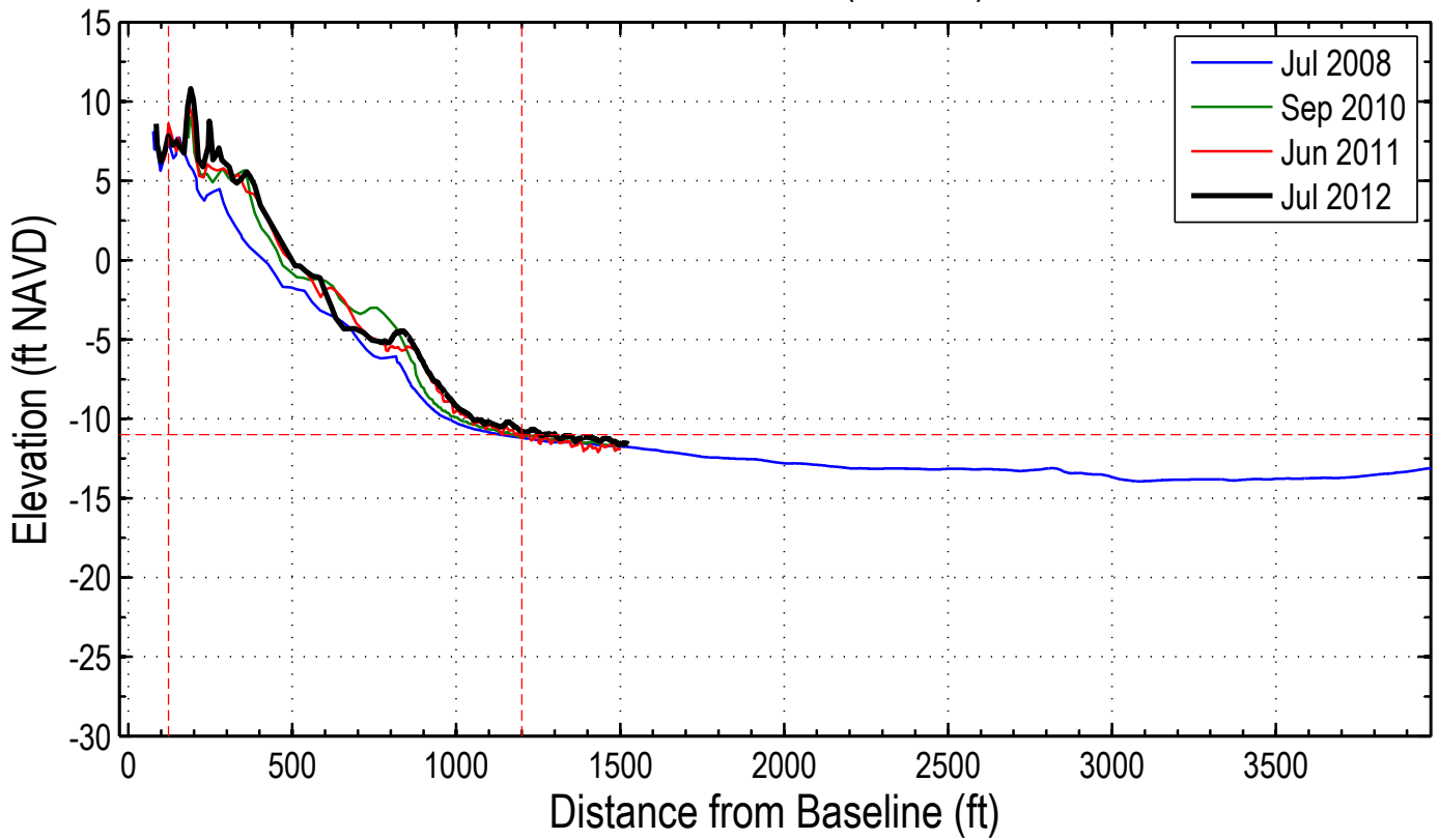
Station: 210+00 (-12+00)
