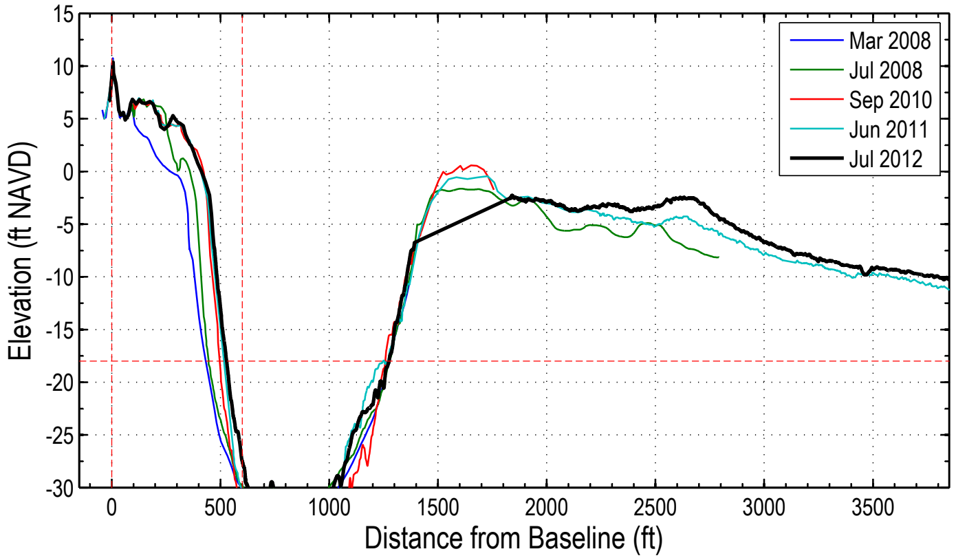
Station: 332+00 (110+00)
