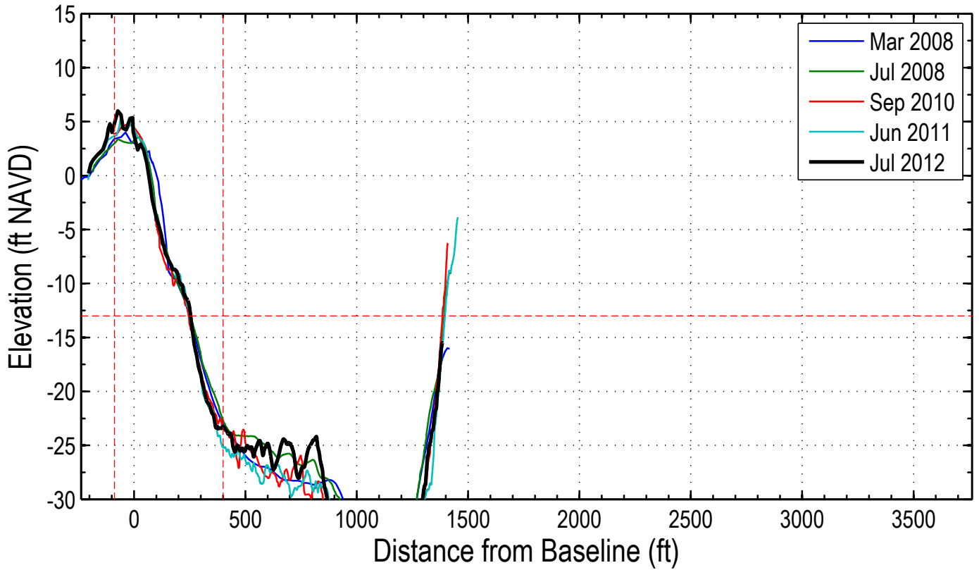
Station: 366+00 (144+00)
