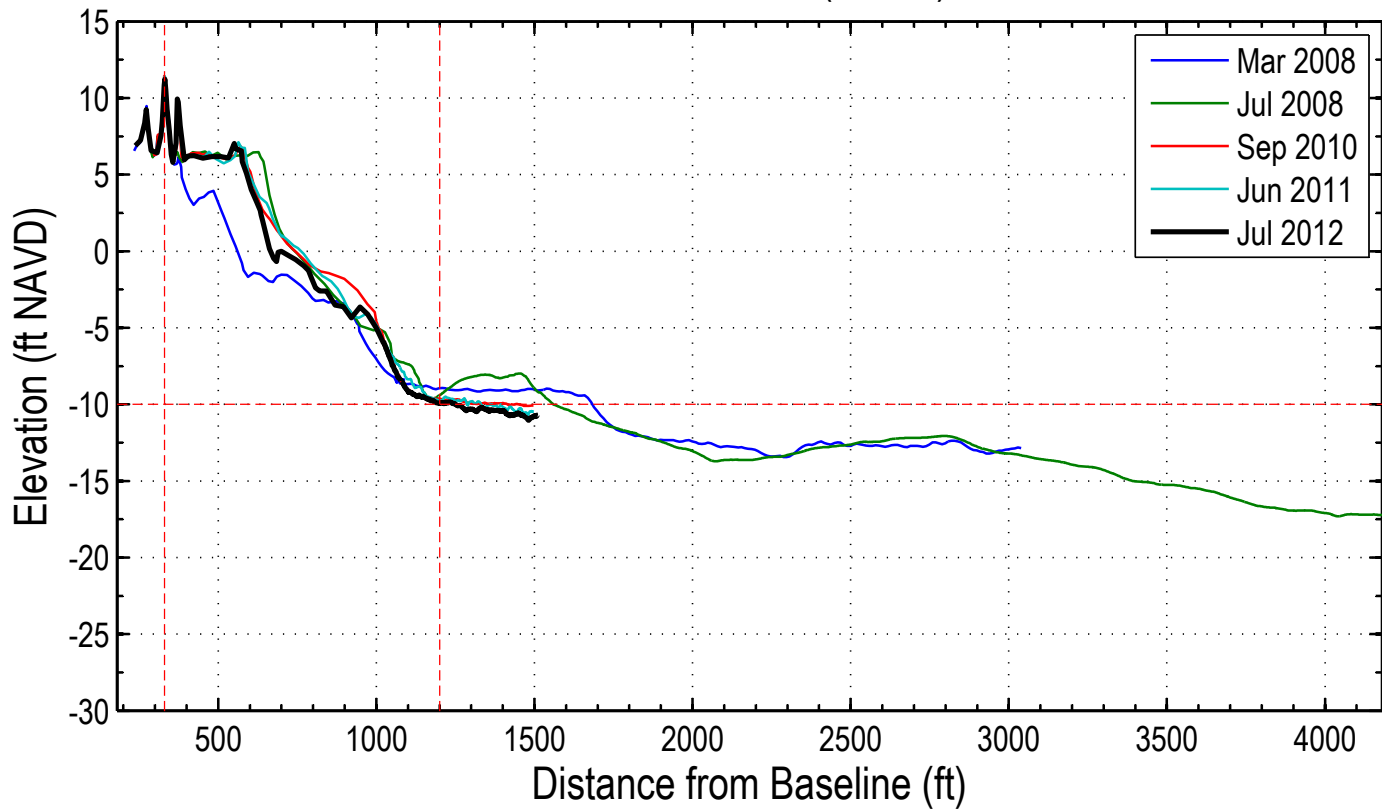
Station: 234+00 (12+00)
