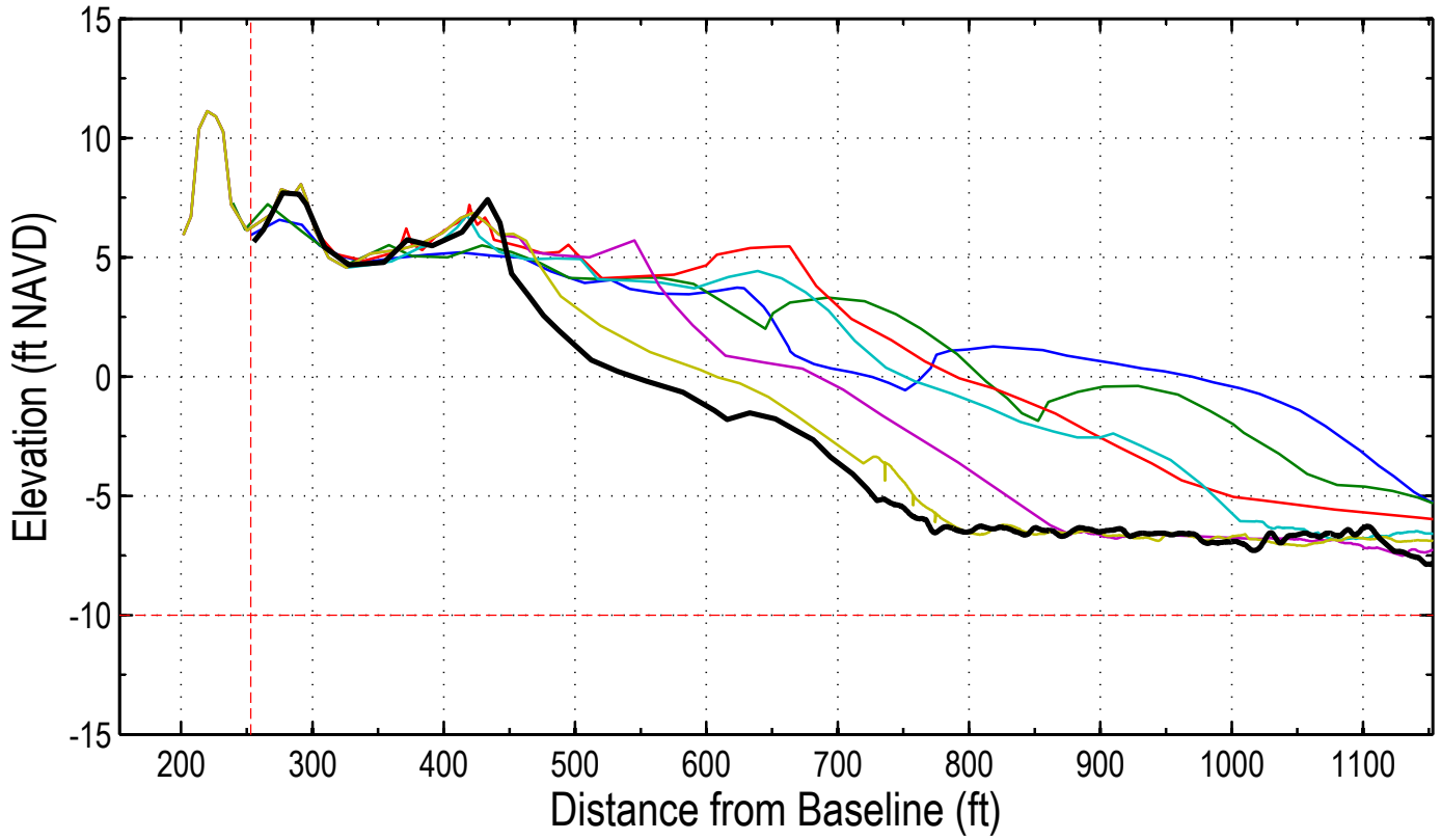
Station: 276+00 (54+00)
