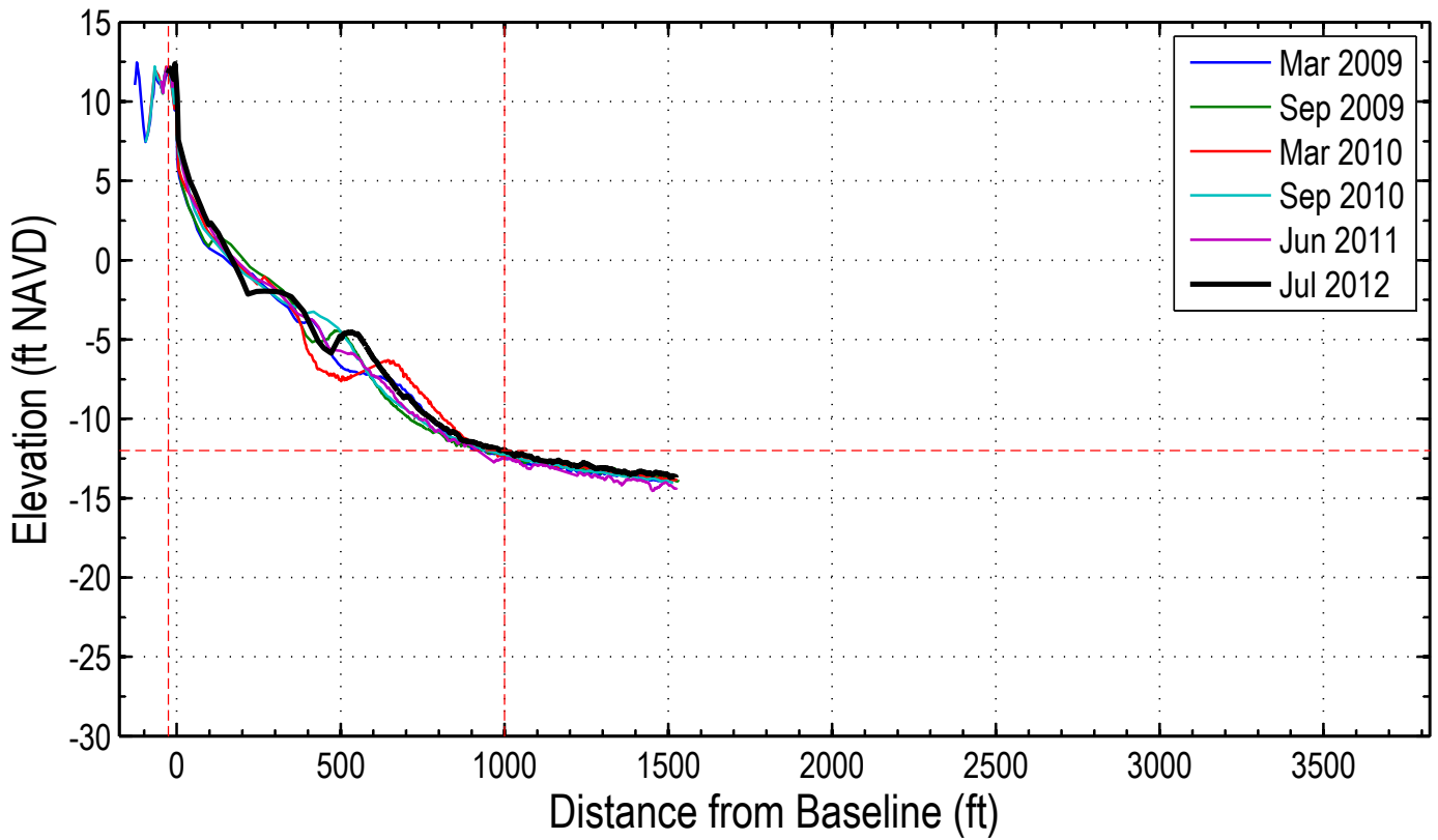
Station: 60+00
