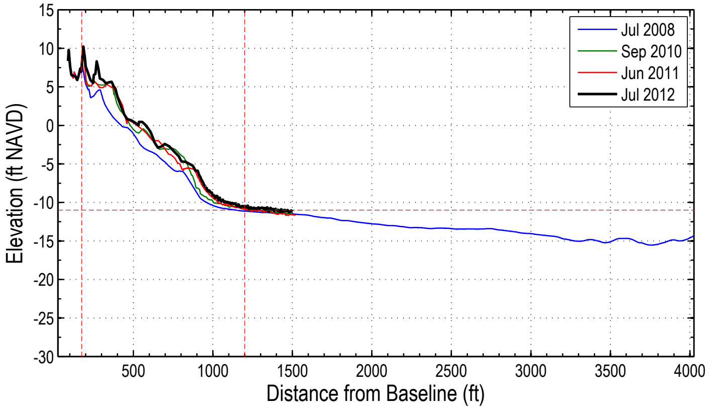
Station: 212+00 (-10+00)
