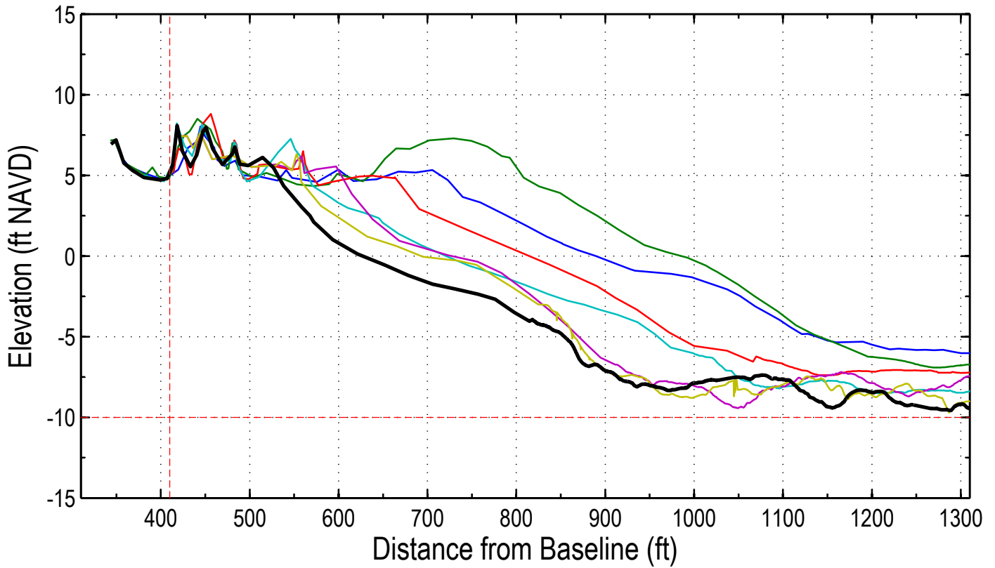
Station: 270+00 (48+00)
