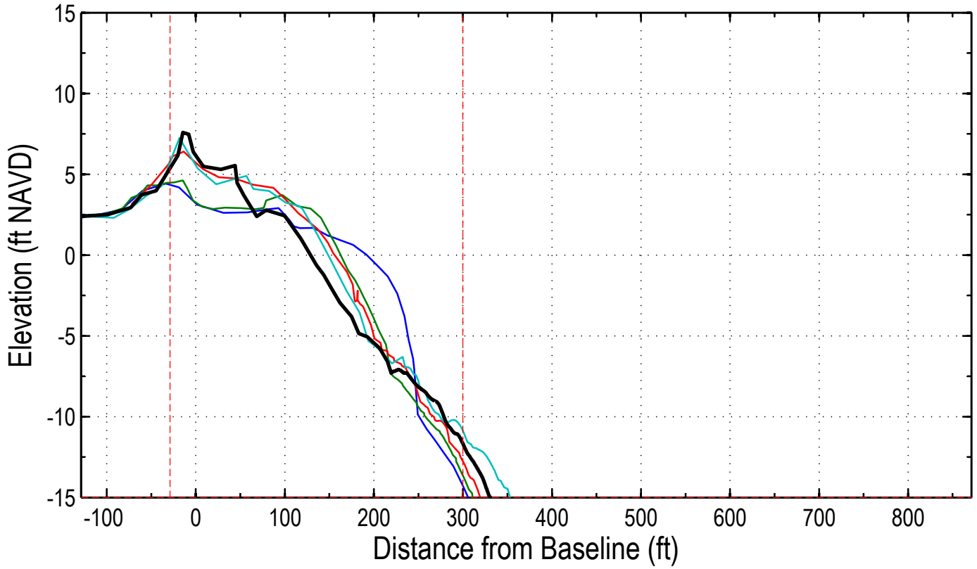
Station: 362+00 (140+00)
