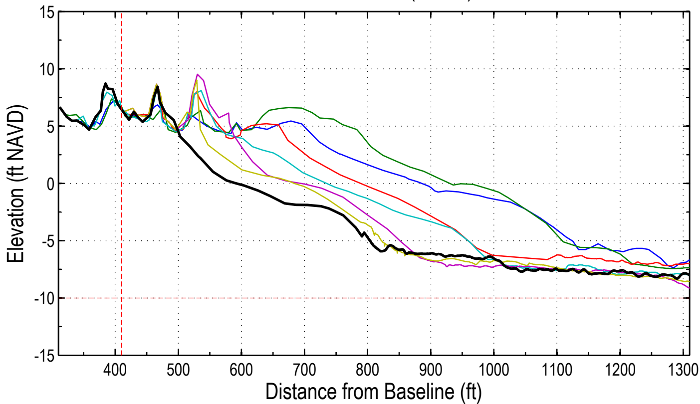
Station: 272+00 (50+00)
