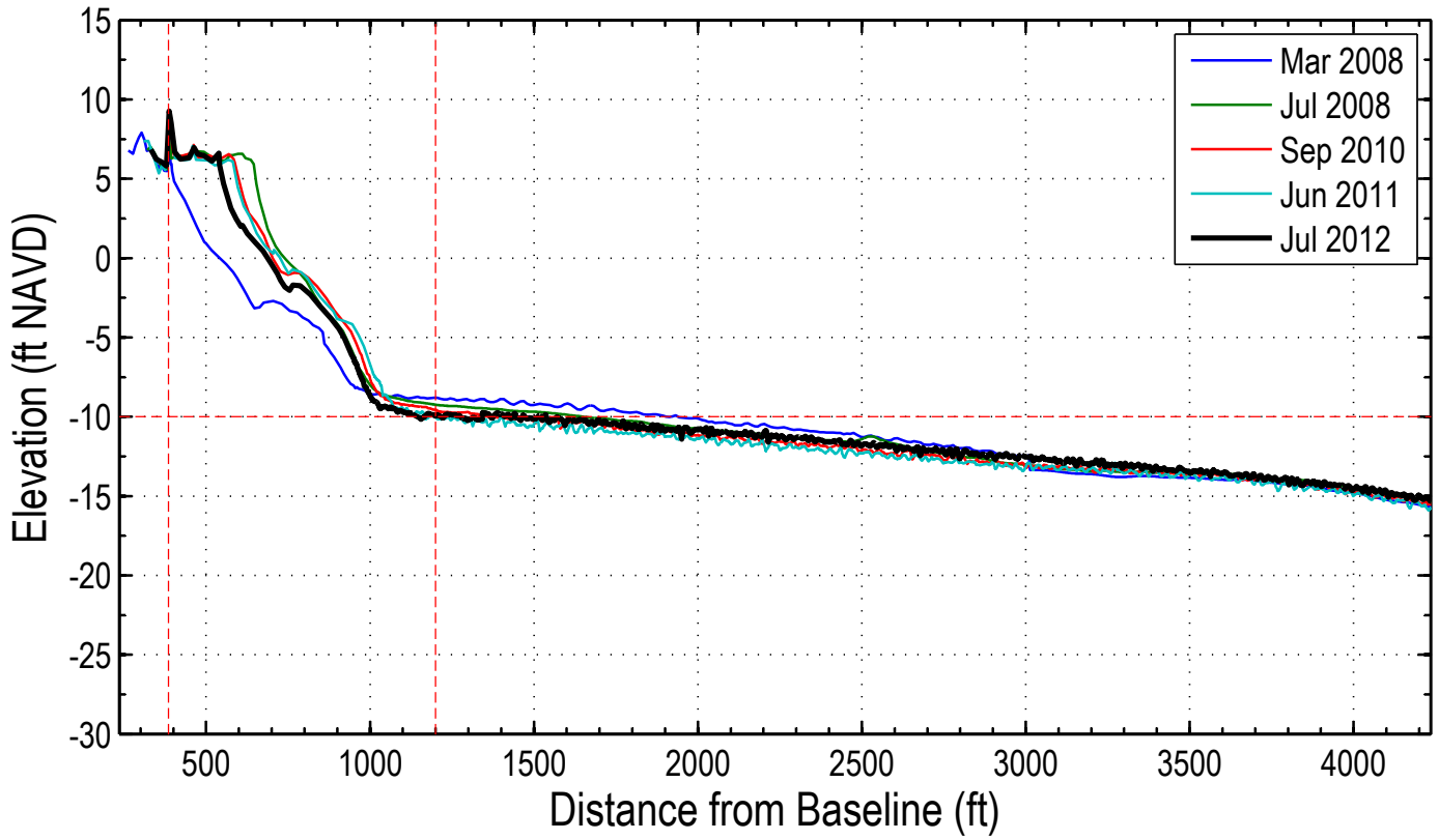
Station: 246+00 (24+00)
