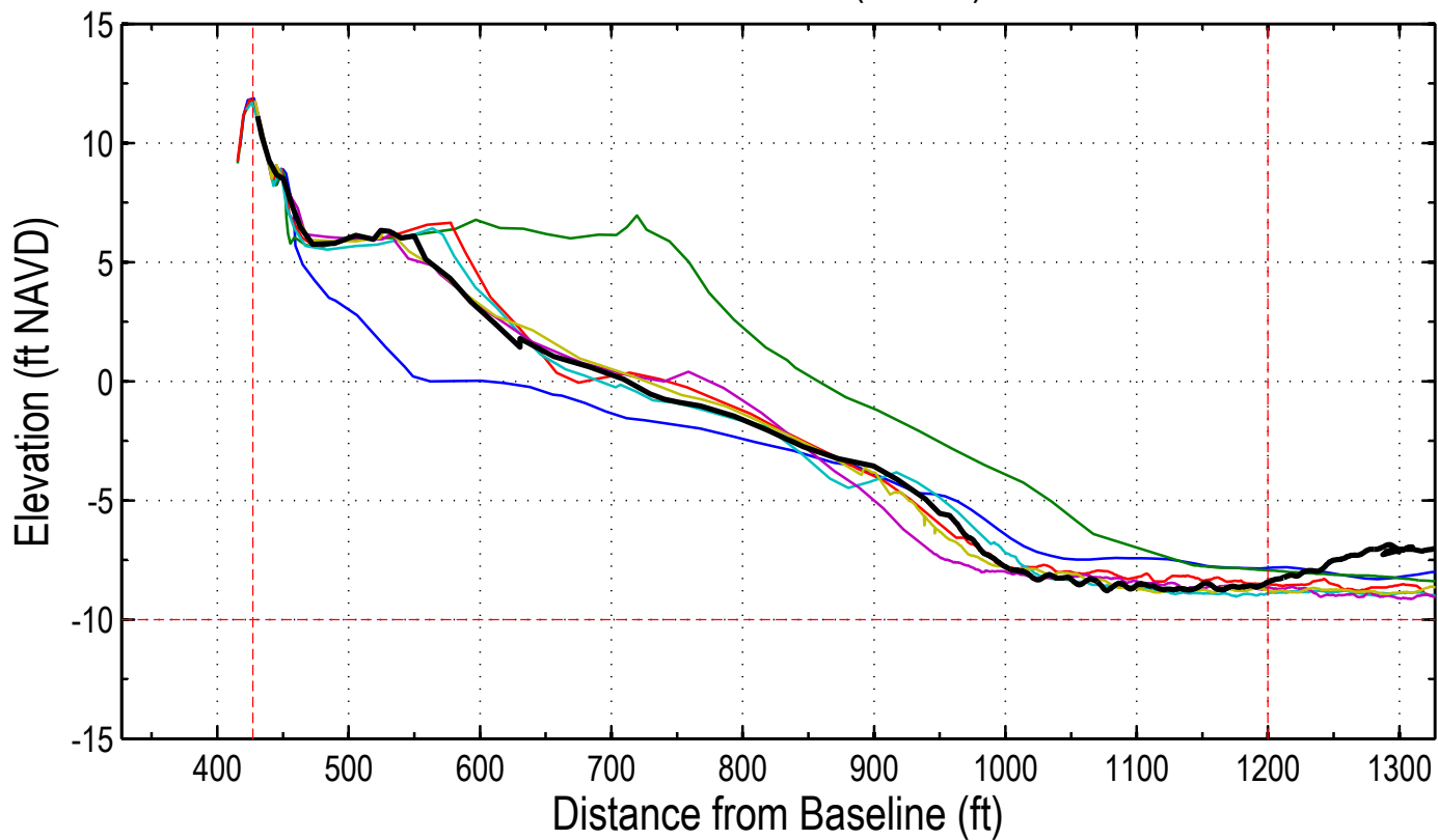
Station: 256+00 (34+00)
