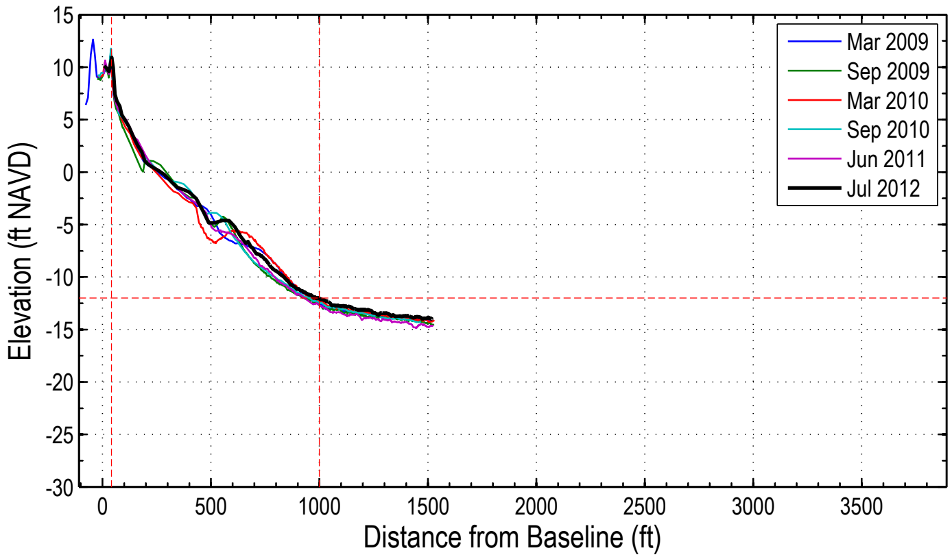
Station: 80+00
