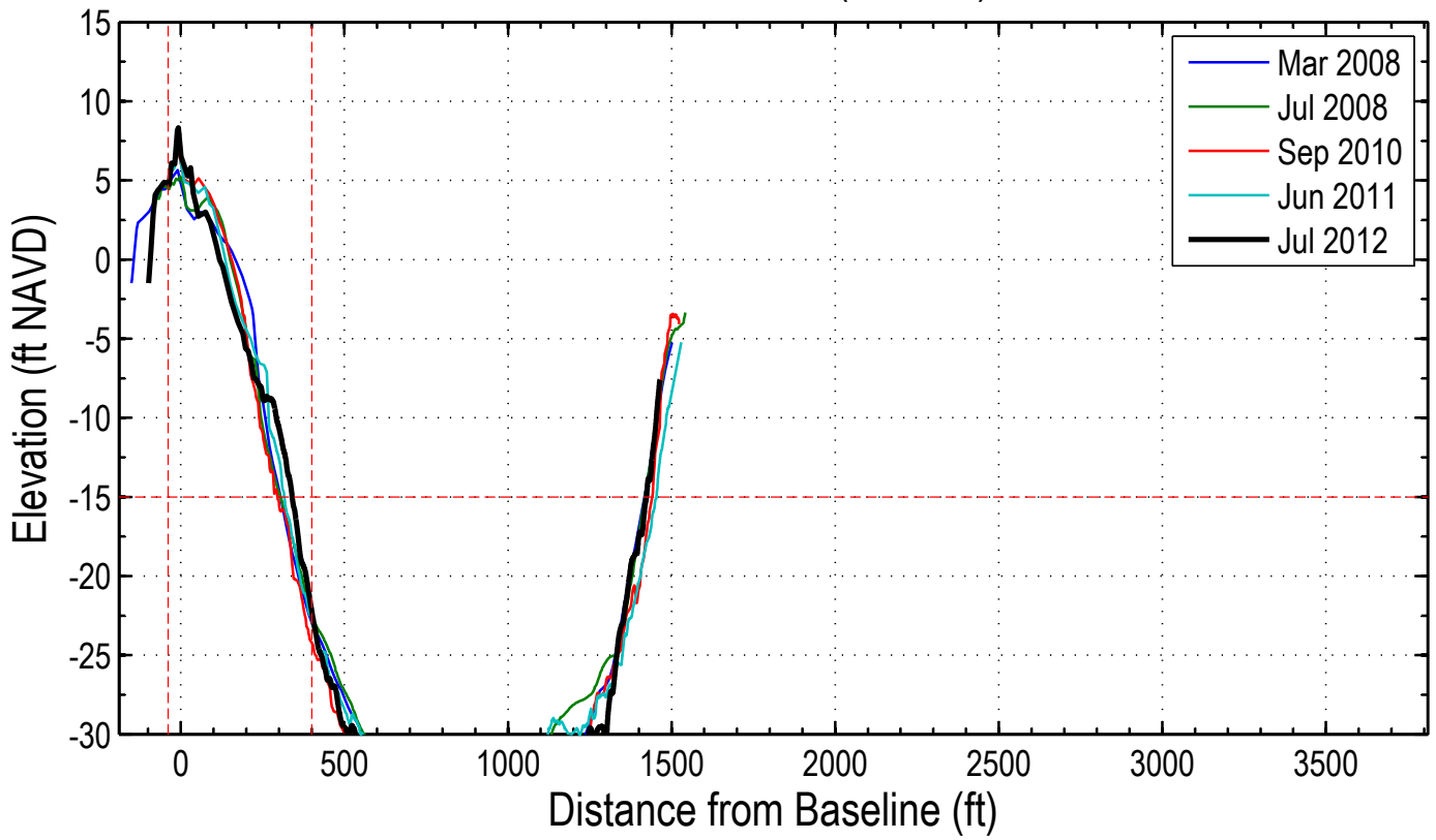
Station: 360+00 (138+00)
