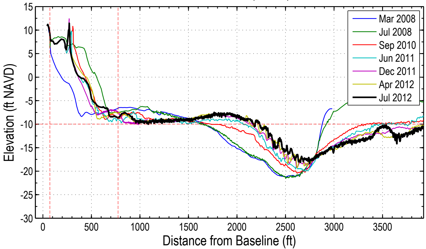
Station: 320+00 (98+00)
