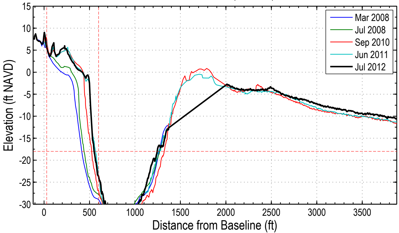
Station: 330+00 (108+00)
