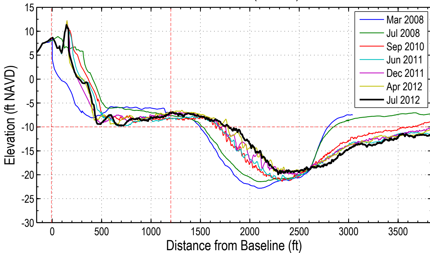
Station: 324+00 (102+00)
