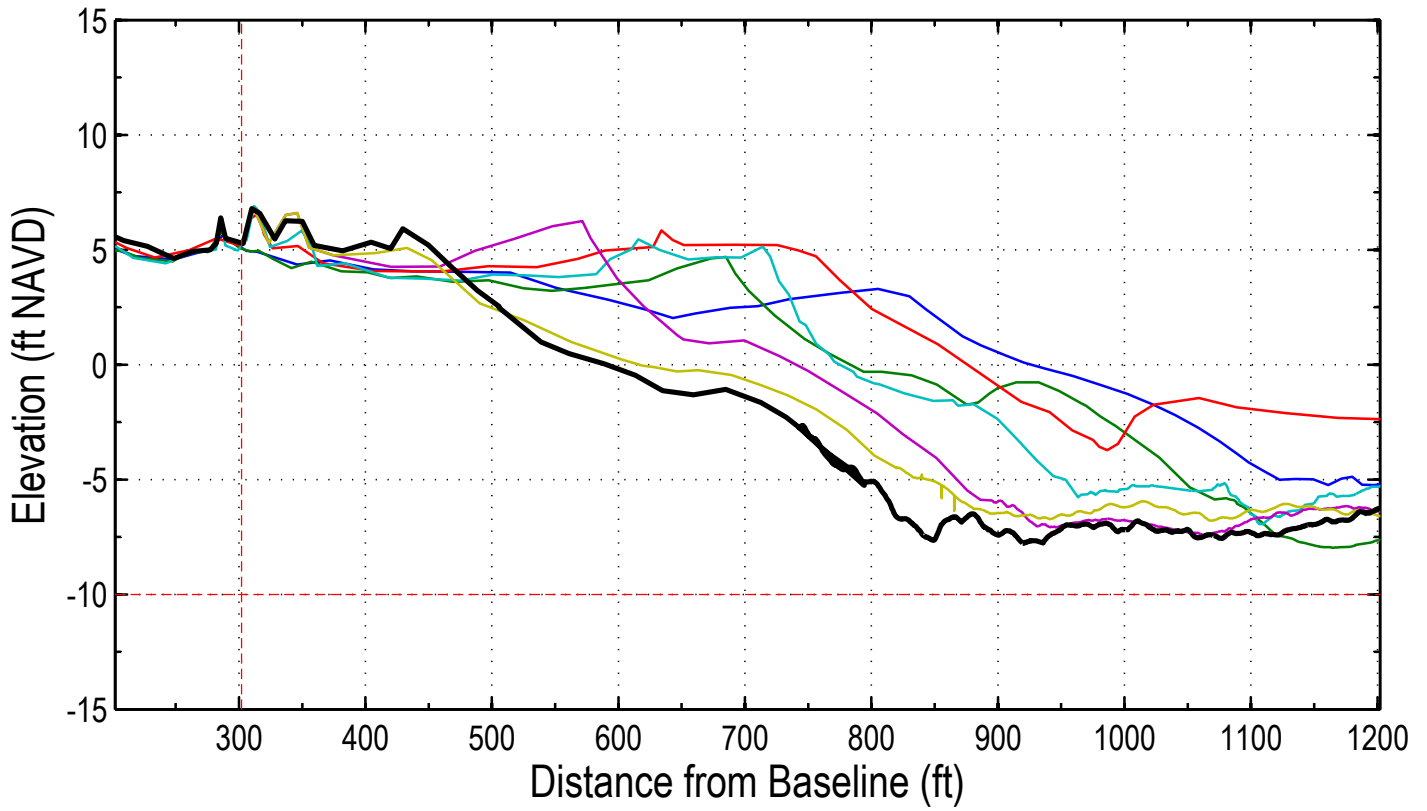
Station: 282+00 (60+00)
