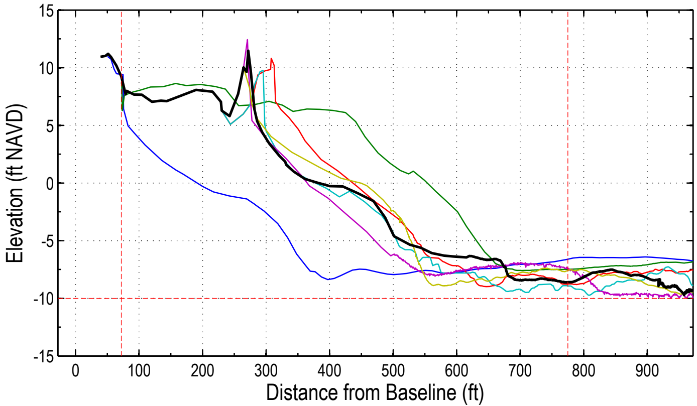
Station: 320+00 (98+00)
