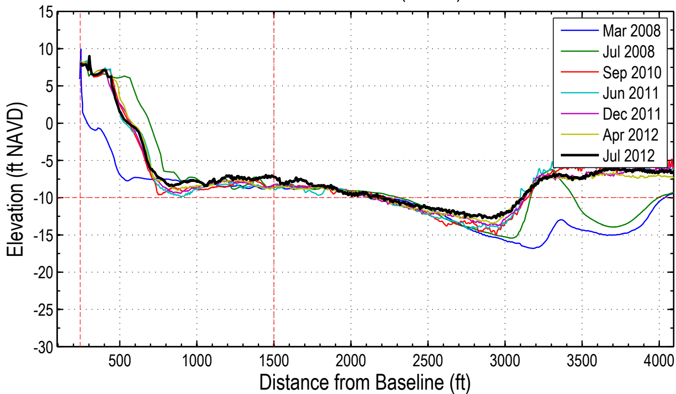
Station: 308+00 (86+00)
